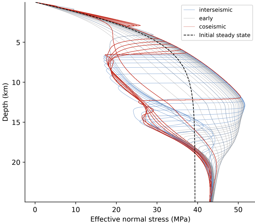
F3b Effective normal stress depth profiles
