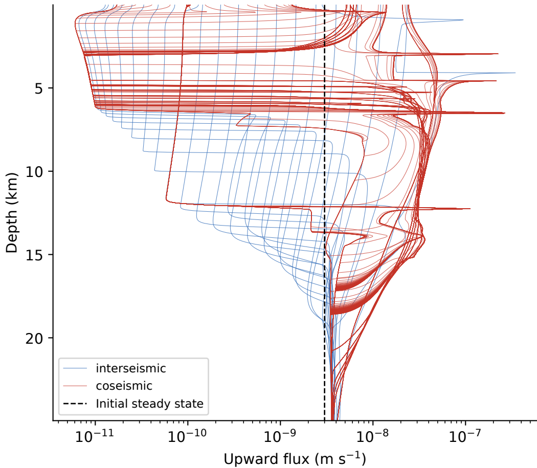
F3f Upward fluid flux depth profiles
