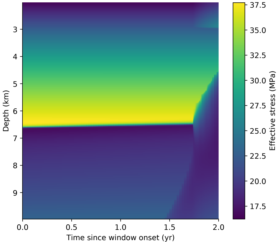
F4c Effective normal stress
