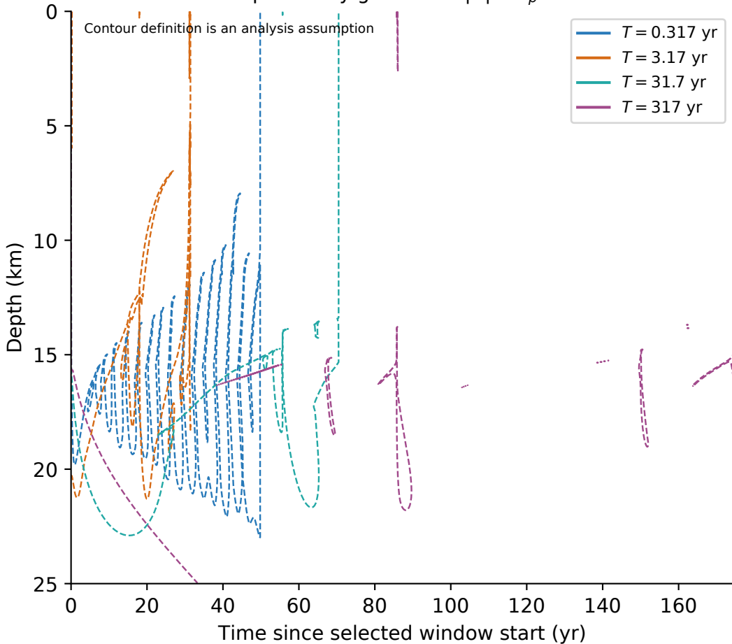
F6: independently generated |V| = V_p contours
