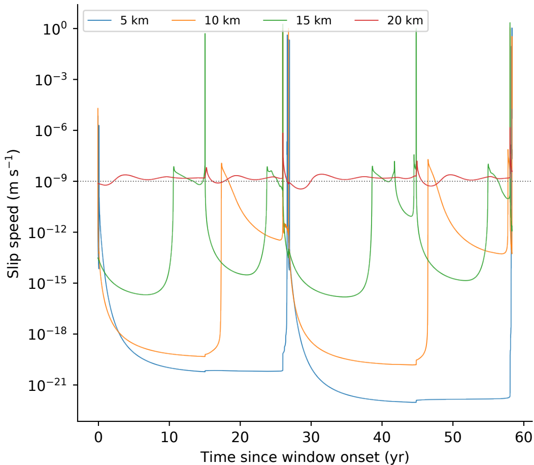
S1a Slip velocity at 5, 10, 15, and 20 km
