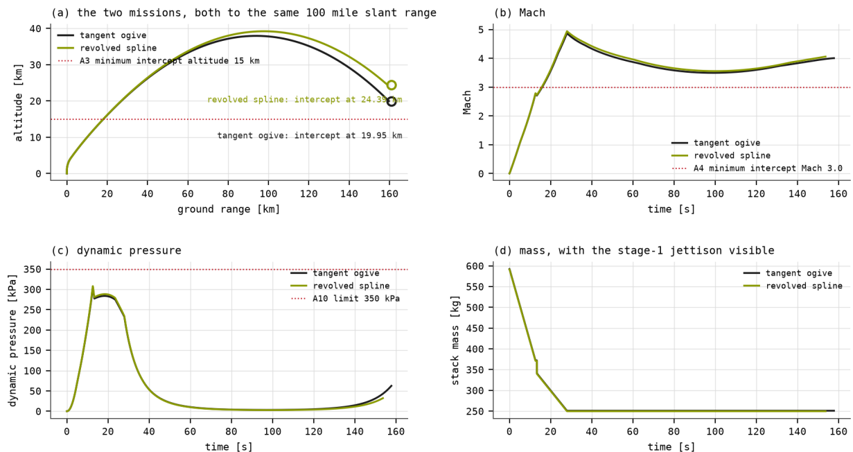
Figure 3. The two flown missions. Both reach the same 100 mile slant range, because that is what the trajectory is flown to. The spline arrives higher, faster and in thinner air.
