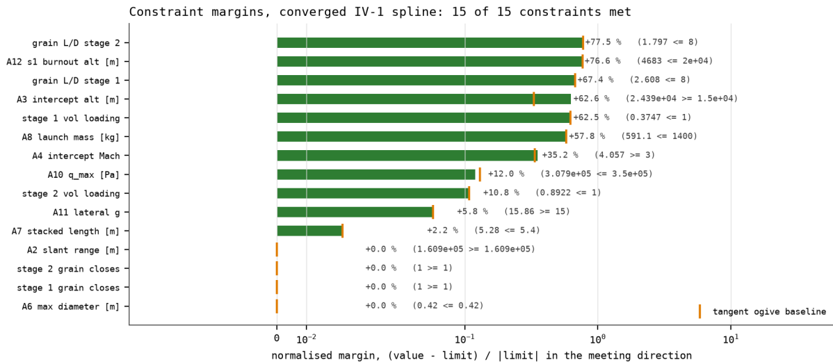
Figure 2. The same margins, drawn. Orange ticks are the tangent-ogive baseline at the same pitchover angle. The two shapes trade margin between A3 and A11.
