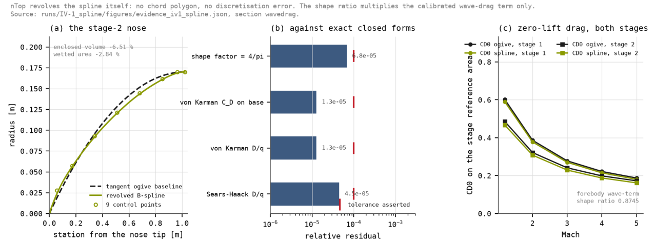
Figure 1. The revolved spline. Panel (a) is the stage-2 nose and the nine control points the notebook computes. Panel (b) is the closed-form validation of the wave-drag model. Panel (c) is the zero-lift drag it moves, in both flight configurations.
