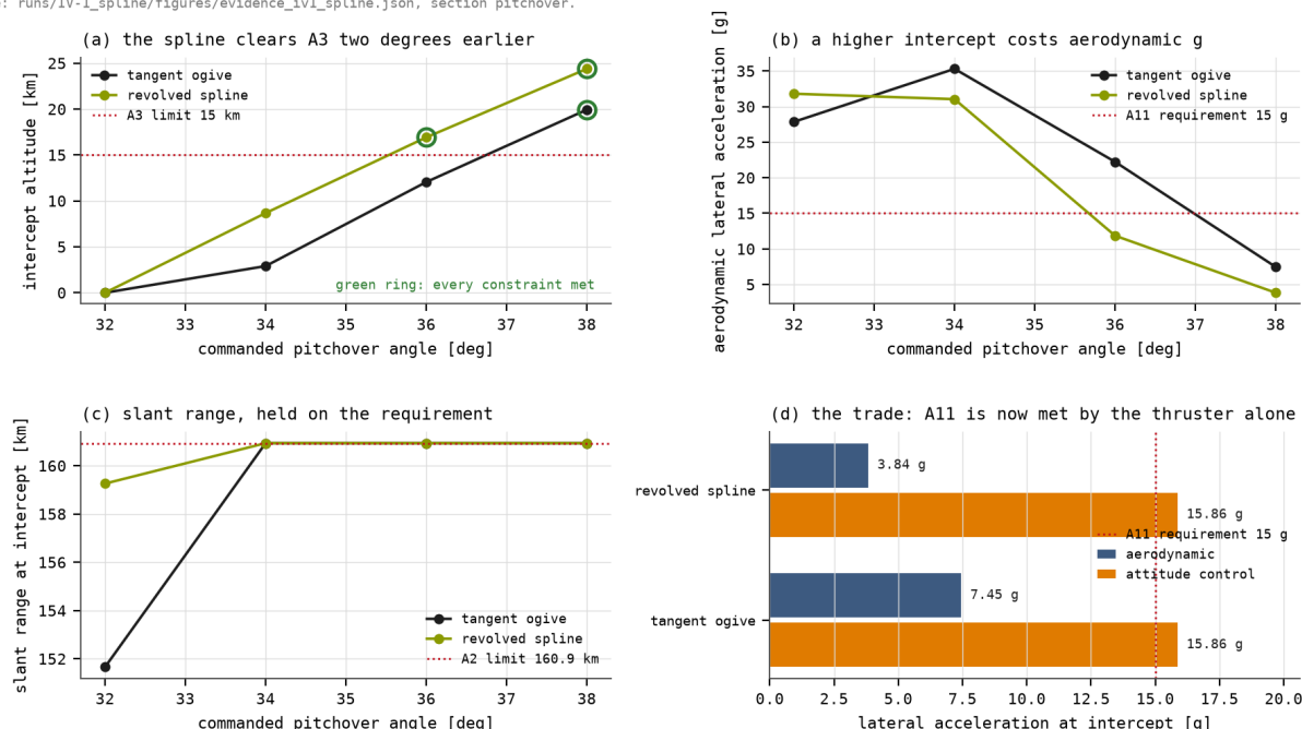
Figure 4. The pitchover sweep. Panel (a) shows the spline clearing A3 two degrees earlier. Panel (b) shows what that costs in aerodynamic g. Panel (d) shows how A11 is actually met at the converged point.
