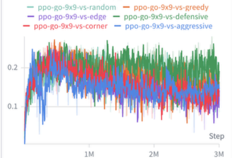
train/clip_fraction
