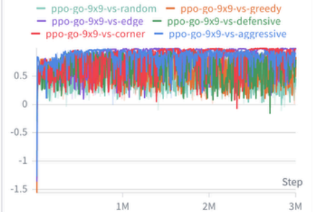
train/explained_var
