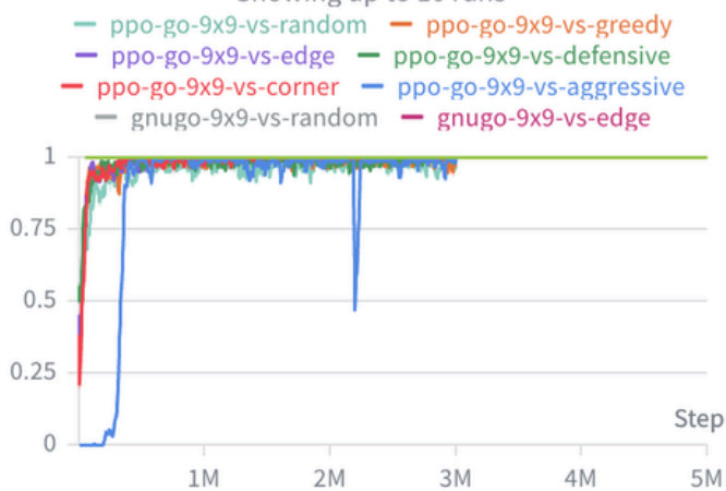
custom/win_rate
