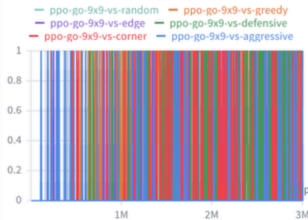
train/early_stopped
