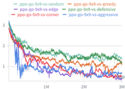
train/entropy
