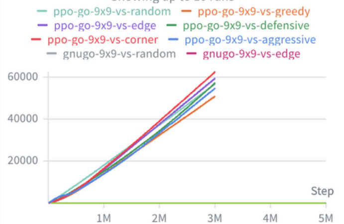
custom/total_episodes
