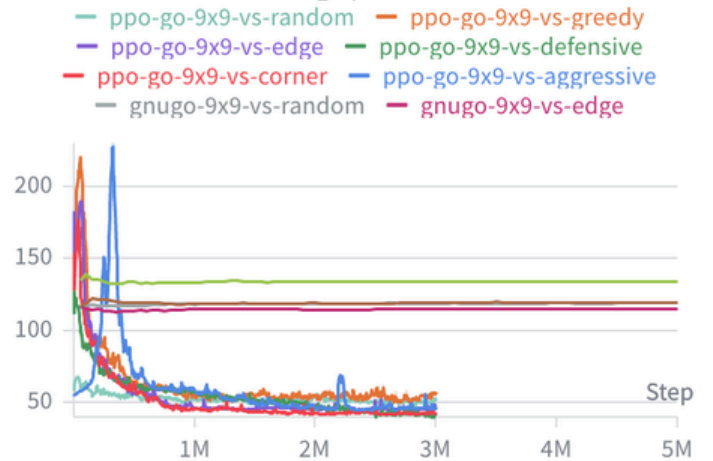
rollout/ep_len_mean
