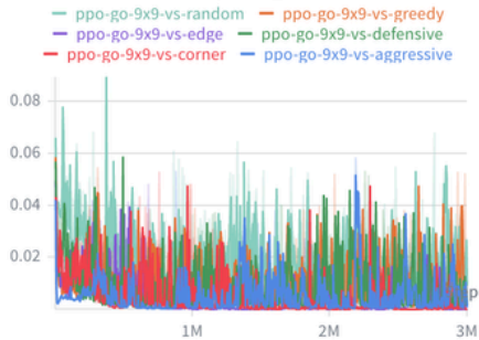
train/value_loss
