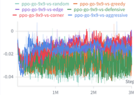
train/policy_loss
