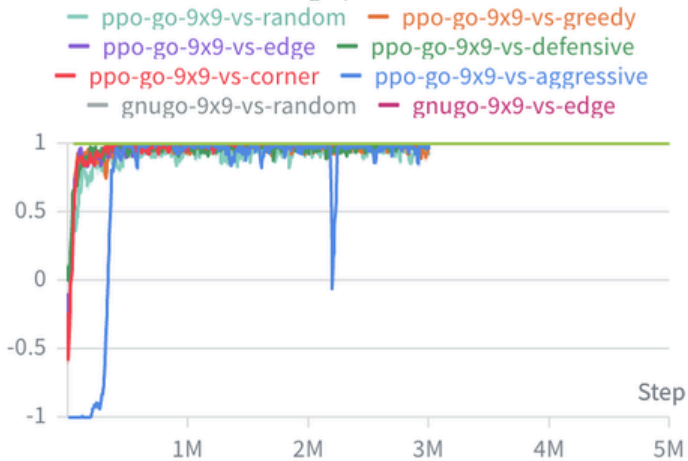
rollout/ep_rew_mean
