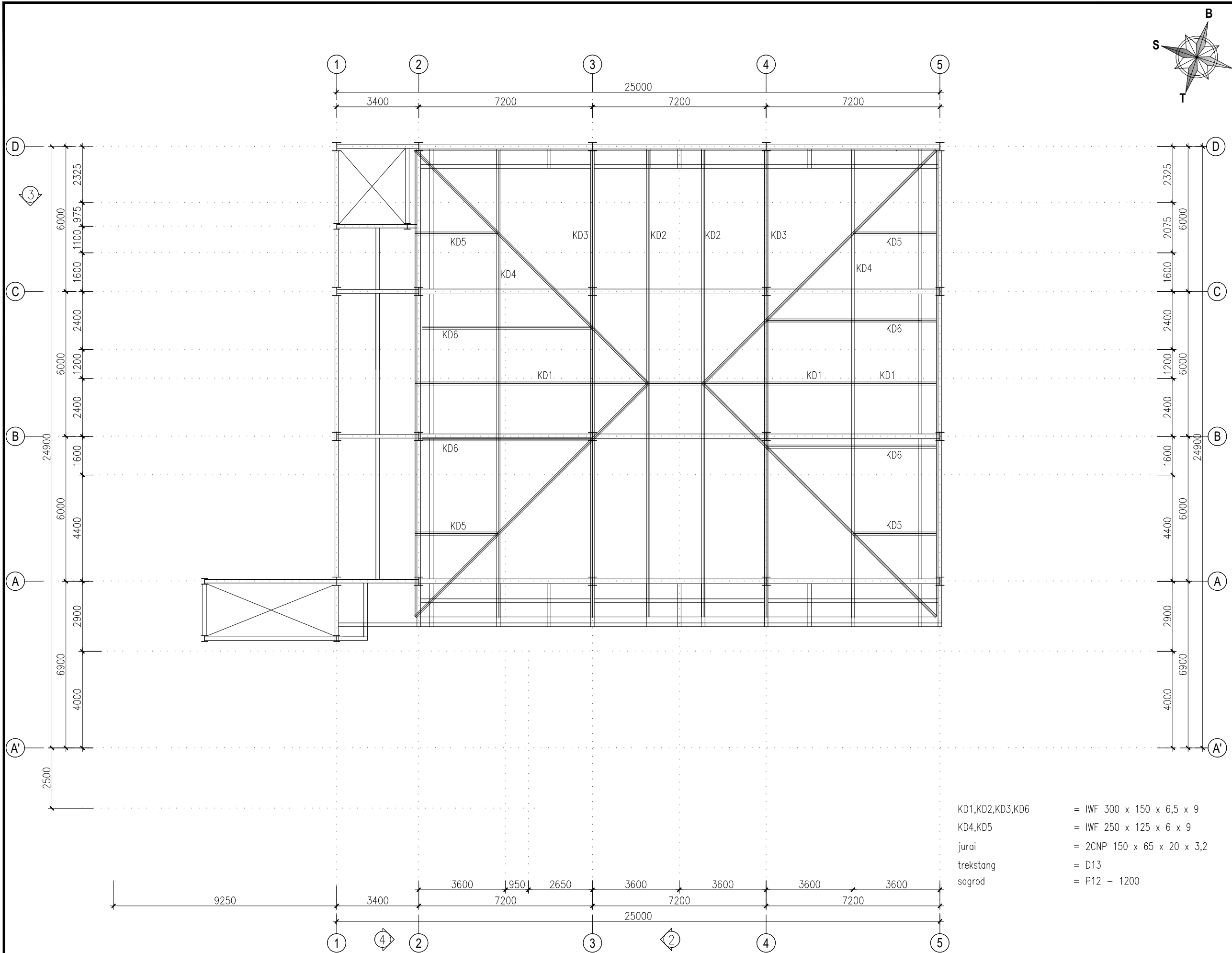
STR DENAH KUDA-KUDA ATAP SKALA 1 : 150
