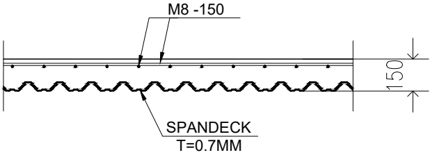
DETAIL PLAT METAL DECK SKALA 1 : 25
