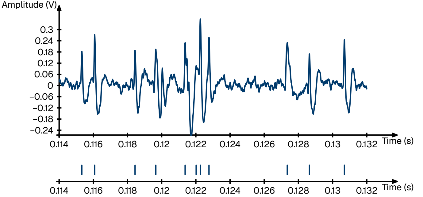
Figure 6: Transformation of continuous membrane voltage (top) into a discrete spike train (bottom). The membrane voltage trace is a recording from the L5 dorsal rootlet of a rat using a multiple electrode array [28]
