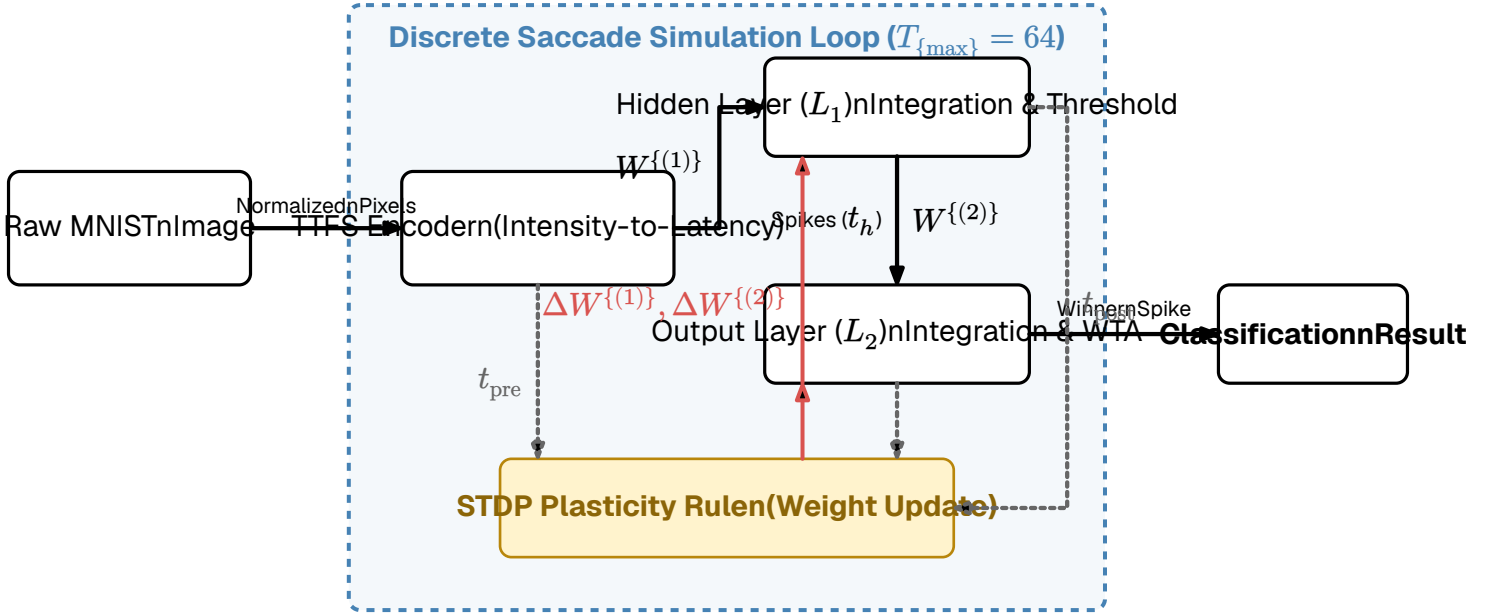
Figure 29: Software architecture and data flow of the Spiking Neural Network (SNN) simulator.
