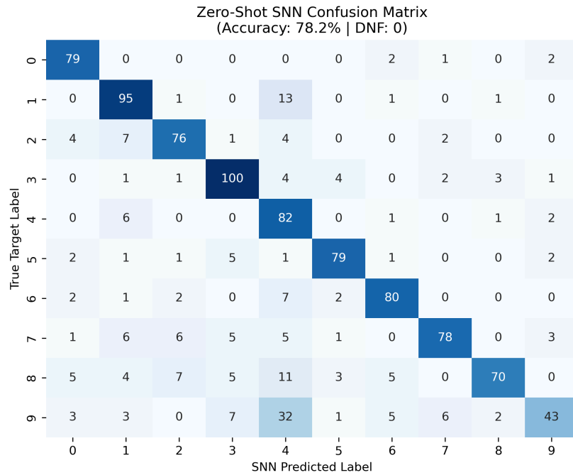
Figure 33: Confusion matrix for the zero-shot SNN on the MNIST test set.
