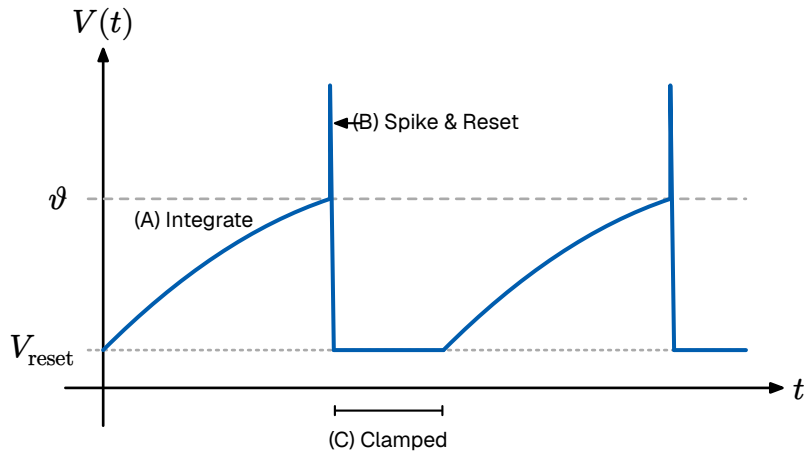
Figure 7: The dynamics of an LIF neuron. (A) The membrane potential integrates inputs. (B) Upon crossing the threshold \vartheta , a spike is emitted and the voltage is reset. (C) The voltage is clamped during the refractory period.
