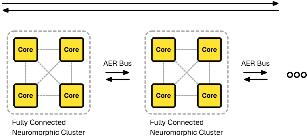
Figure 21: Hierarchical routing in neuromorphic hardware. Address-Event Representation (AER) buses handle sparse, long-distance communication between neuron clusters, while local, intra-cluster communication relies on dense physical wiring.
