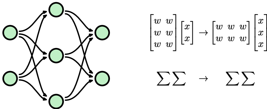
Figure 19: Deep learning as matrix multiplication. Forward and backward passes rely on dense matrix products, necessitating high-bandwidth memory access.
