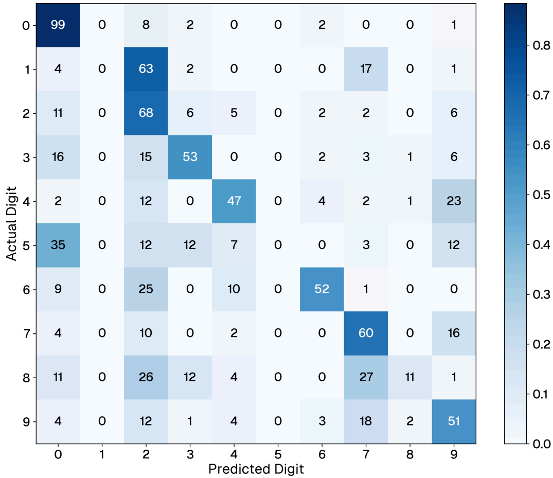
Figure 36: Confusion matrix for the unsupervised STDP network. While primary classes are successfully clustered, the network struggles with overlapping topologies (e.g., classifying ‘5’s as ‘0’s) due to the holistic nature of the learned templates. The STDP trained network fails to classify any number that is ‘5’ or ‘1’.
