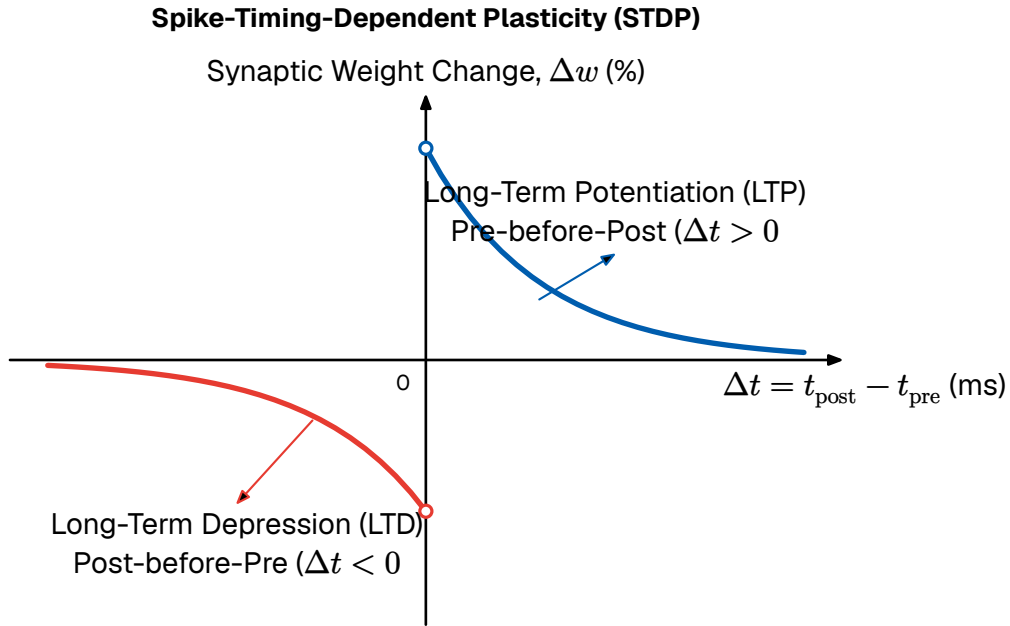
Figure 16: The Spike-Timing-Dependent Plasticity (STDP) Learning Curve. Synaptic weight change is plotted against spike timing difference. Pre-before-post timing triggers strengthening (Long-Term Potentiation (LTP)), while post-before-pre triggers weakening (Long-Term Depression (LTD)).
