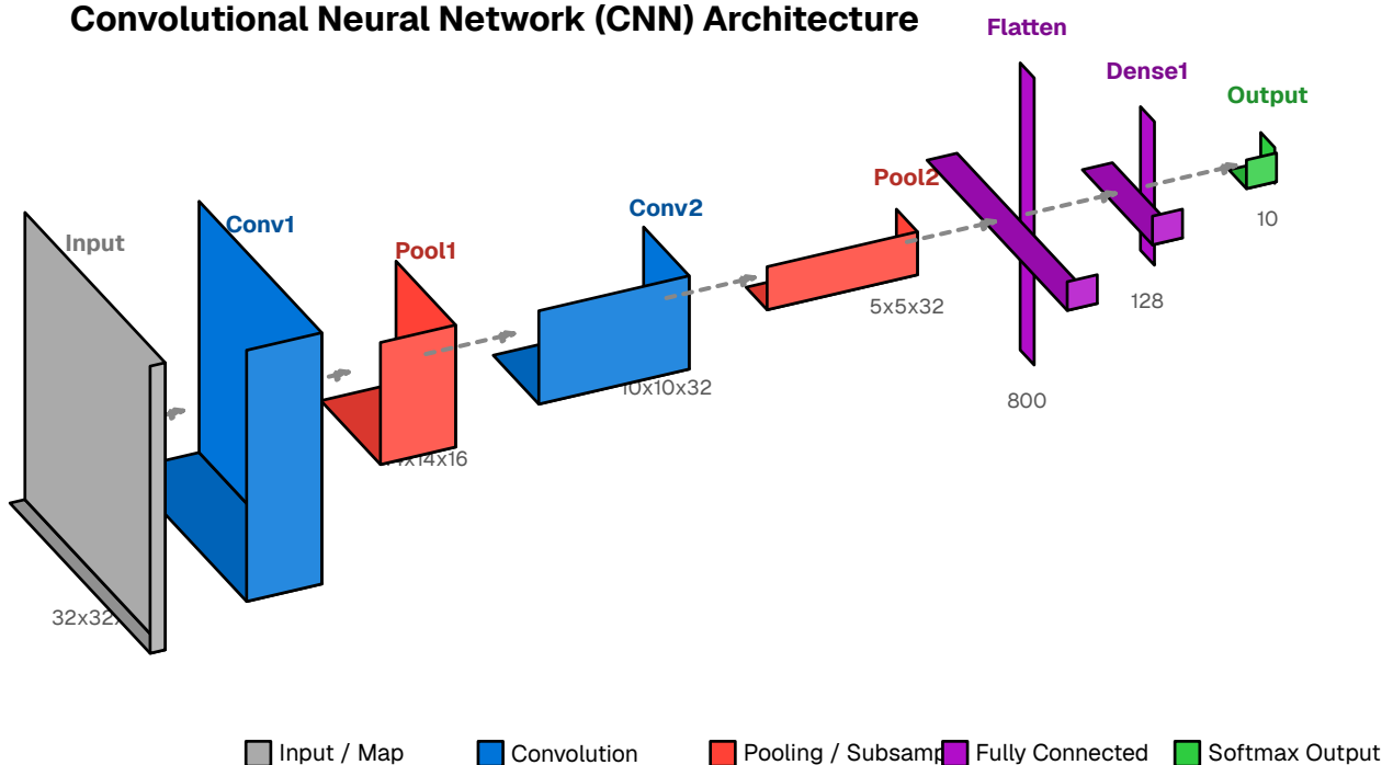
Figure 33: Network architecture for the task at hand
