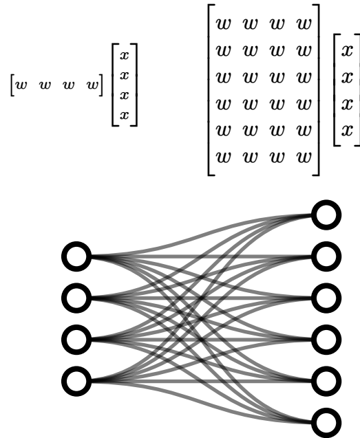
Figure 28: Deep Learning as Matrix Multiplication. Both forward and backward passes rely on dense matrix-vector products, necessitating high-bandwidth memory access.
