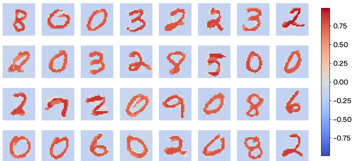
Figure 33: Hidden layer receptive fields ( W_1 ) after unsupervised STDP training. The hard WTA competition forces Vector Quantization, resulting in recognizable, holistic templates of entire digits.
