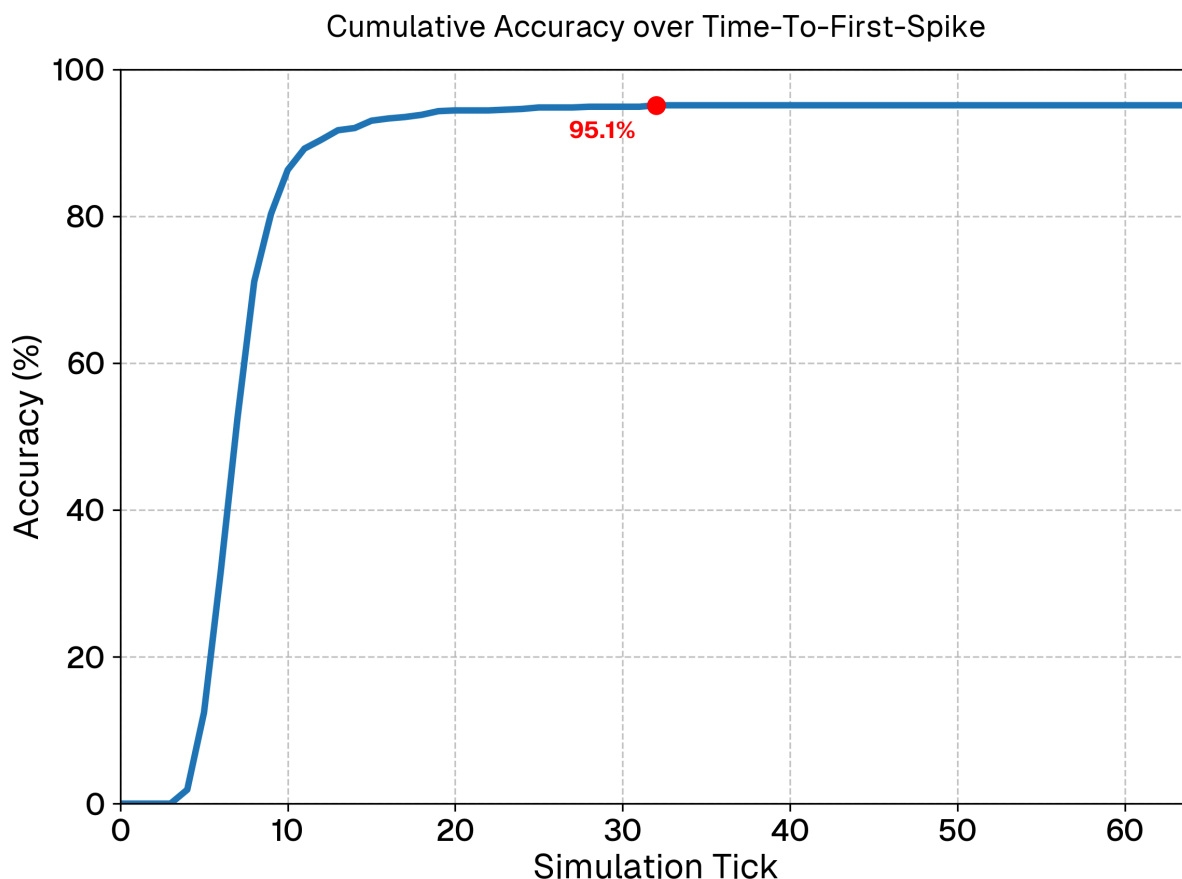
Figure 31: Cumulative classification accuracy over the 64-tick temporal window. Accuracy follows a sigmoid-like “S-curve,” showing that the majority of correct classifications are finalized early in the saccade.
