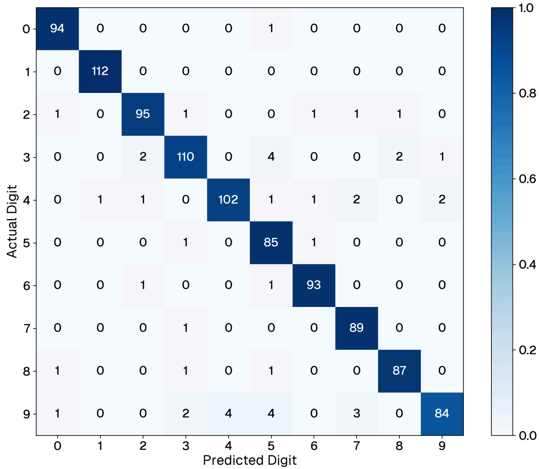
Figure 32: Confusion matrix for the zero-shot SNN on the MNIST test set. The strong diagonal indicates the temporal integration preserved the original ANN decision boundaries.
