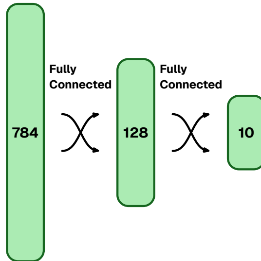
Figure 25: Network architecture. The 28x28 images are flattened and passed through a Fully Connected Network. Both the Artificial Neural Network (ANN) and Spiking Neural Network (SNN) share this identical macroscopic topology.
