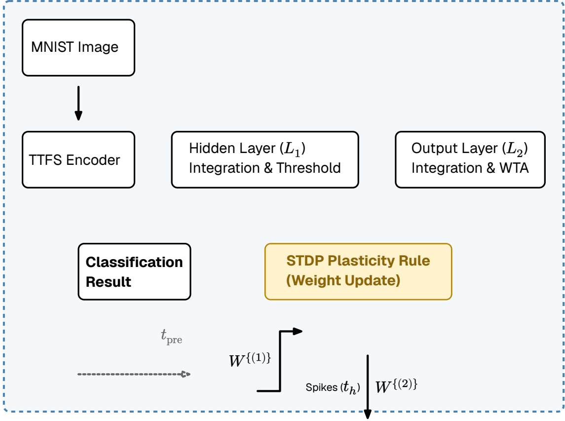
Figure 29: Software architecture and data flow of the Spiking Neural Network (SNN) simulator.
