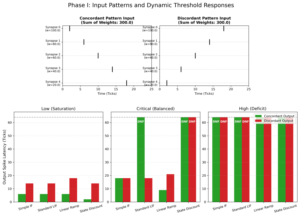
Figure 30: Input spike distributions and resulting temporal dynamics across the three threshold regimes.
