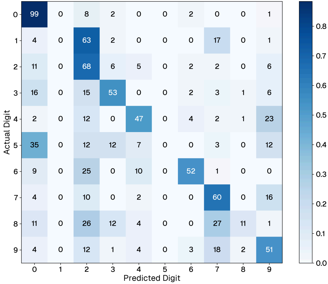
Figure 35: Confusion matrix for the unsupervised STDP network. While primary classes are successfully clustered, the network struggles with overlapping topologies (e.g., classifying ‘4’s as ‘9’s) due to the holistic nature of the learned templates.
