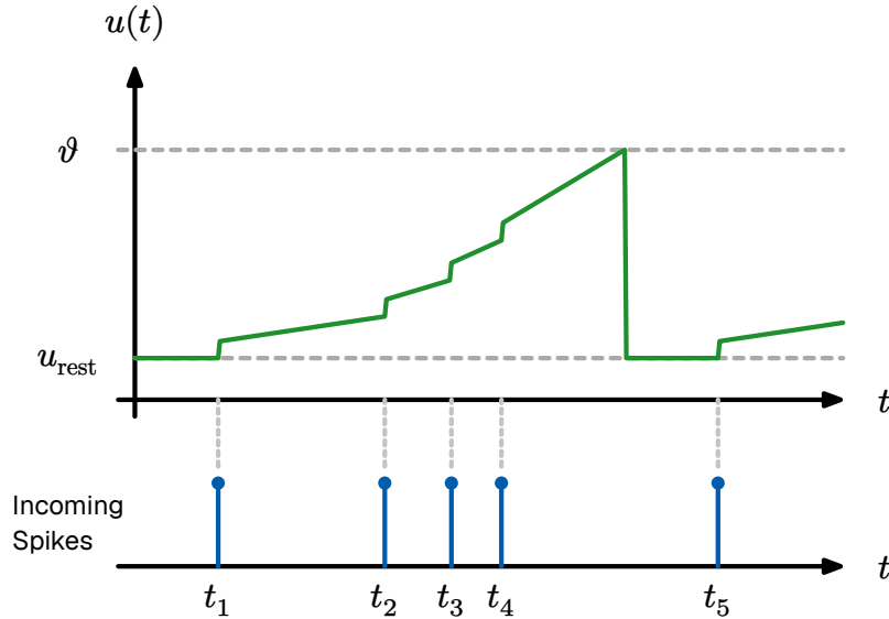
Figure 29: Evolution of state variables in Model C. This demonstrates the resulting piecewise linear membrane potential u(t) . Note how earlier spikes increase the integration gradient, accelerating the trajectory toward the firing threshold \theta .
