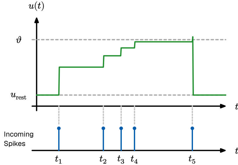
Figure 30: Evolution of state variables in Model D. This demonstrates a neuron model where new incoming spikes have an exponentially decaying influence based on the current potential u(t) .
