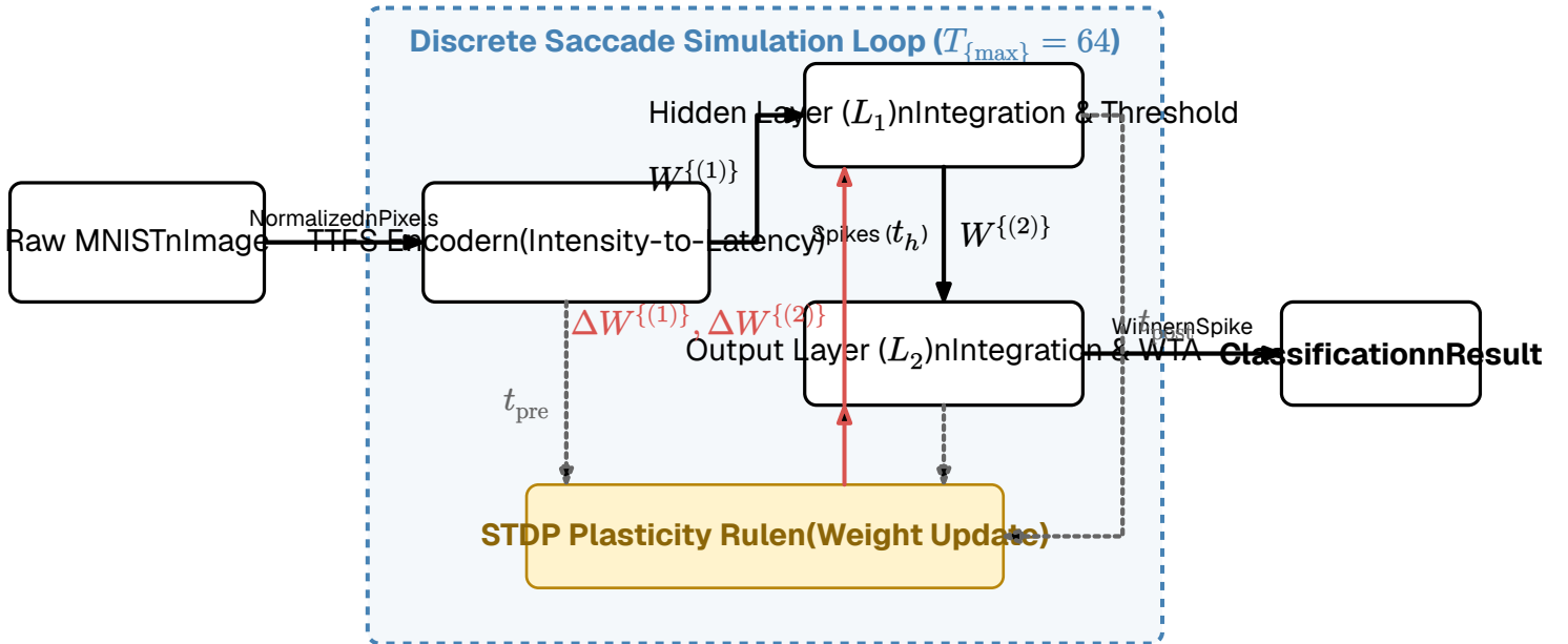
Figure 27: Software architecture and data flow diagram of the spiking neural network simulator. The diagram illustrates the pipeline from raw MNIST images to temporal spikes, the core event-driven simulation loop, and the local plasticity feedback mechanism.
