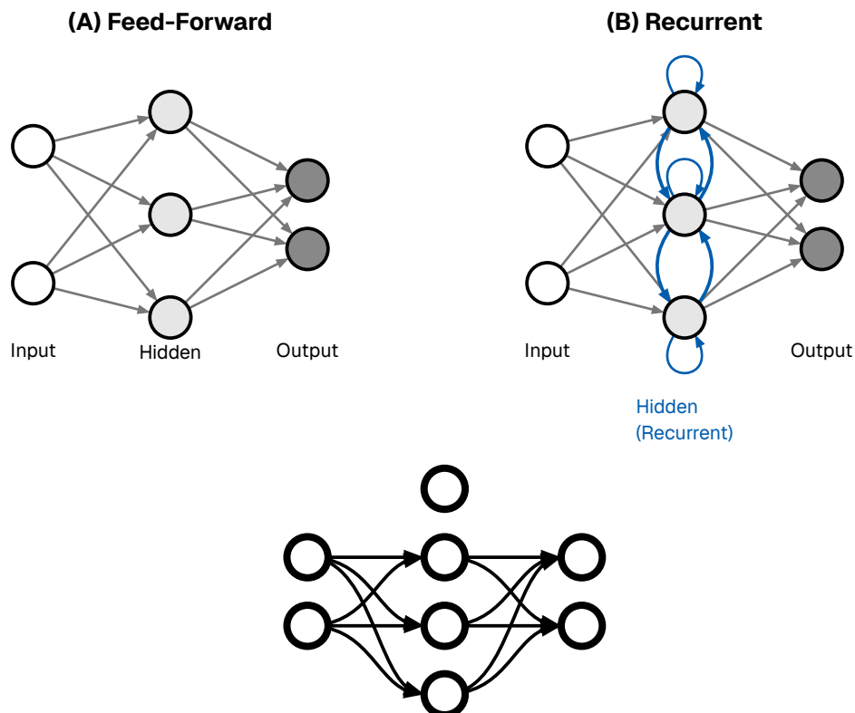
Figure 14: Network topologies. (A) Feed-Forward. (B) Recurrent.
