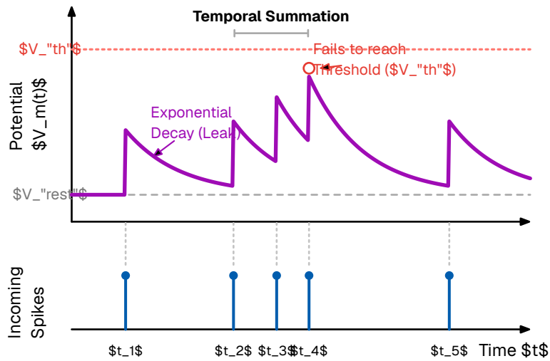
Figure 28: Neuron model where new incoming spikes have an exponentially decaying influence based on the current potential.
