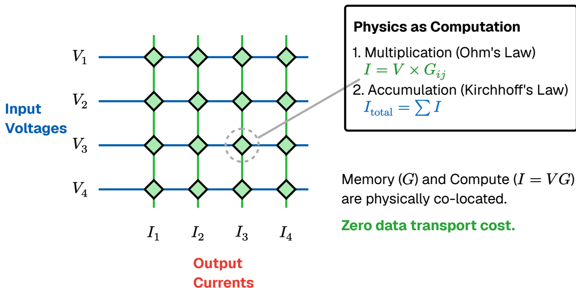
Figure 21: In-Memory Computing via a Crossbar Array. Unlike von Neumann architectures, memory and computation are physically co-located. Input voltages ( V ) are applied to the wordlines. Memory elements at the junctions hold programmable conductances ( G ). Multiplication is natively performed at each junction by Ohm's Law ( I = V \times G ), and resulting currents are summed along the bitlines via Kirchhoff's Current Law. This allows dense matrix-vector multiplications to occur in a single analog time step with zero data transport cost.
