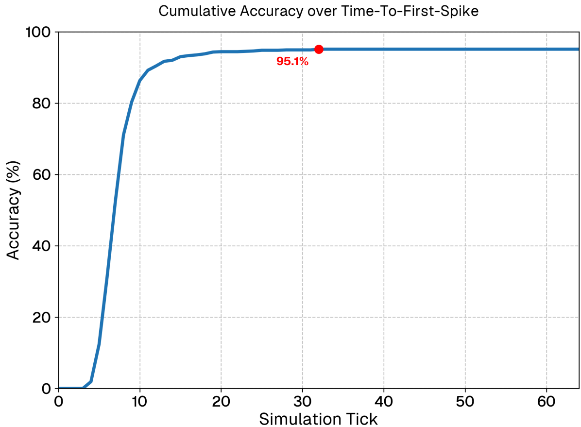
Figure 31: Cumulative classification accuracy over the 64-tick temporal window. Accuracy follows a sigmoid-like S-curve, showing that the majority of correct classifications are finalized early in the saccade.
