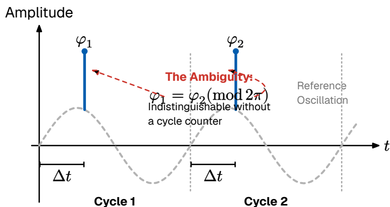
Figure 14: The phase ambiguity problem in temporal encoding. Spikes occurring at the same relative phase ( \varphi_1 and \varphi_2 ) across different oscillation cycles are mathematically indistinguishable ( \varphi_1 = \varphi_2 (\text{mod } 2\pi) ). Without a mechanism to track the global cycle count, downstream neurons cannot determine whether a spike represents a delayed response to a previous stimulus or an early response to a new one.
