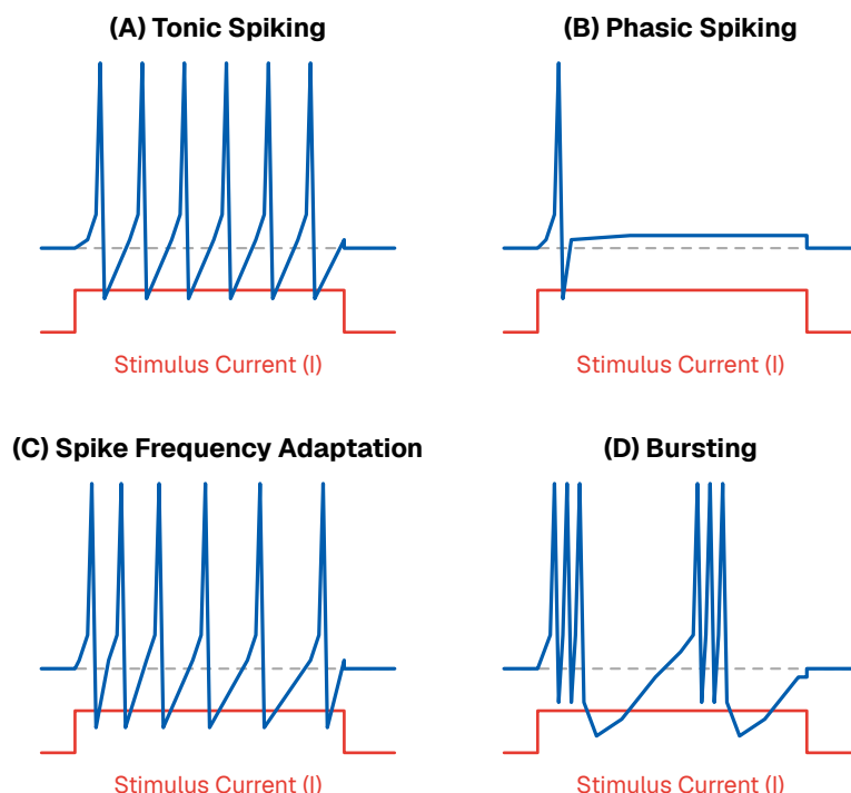
Figure 10: The Generalized LIF model is capable of reproducing the diverse firing patterns of biological cortical neurons, as categorized by Izhikevich (2003) [1].
