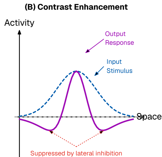
Figure 18: The mechanism of lateral inhibition. (A) A highly stimulated neuron in the input layer strongly excites its corresponding output neuron while simultaneously sending lateral inhibitory signals to its immediate neighbors. (B) This architectural motif acts as a spatial filter, producing a contrast enhancement effect. A broad input stimulus (dashed blue line) is transformed into a sharper output response (solid purple line) characterized by an amplified center and suppressed surroundings (a “Mexican hat” profile), thereby sharpening signal boundaries.
