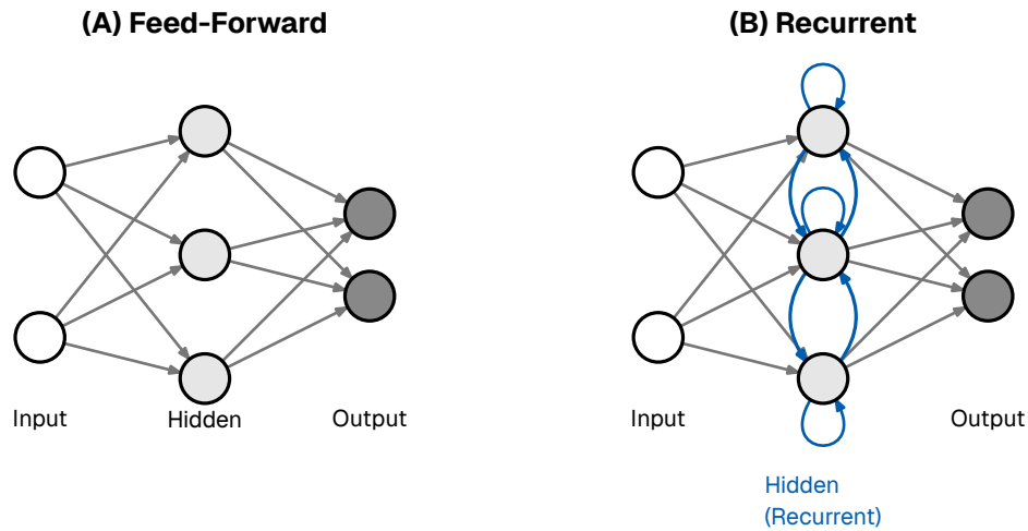
Figure 16: Network topologies. (A) Feed-Forward. (B) Recurrent.
