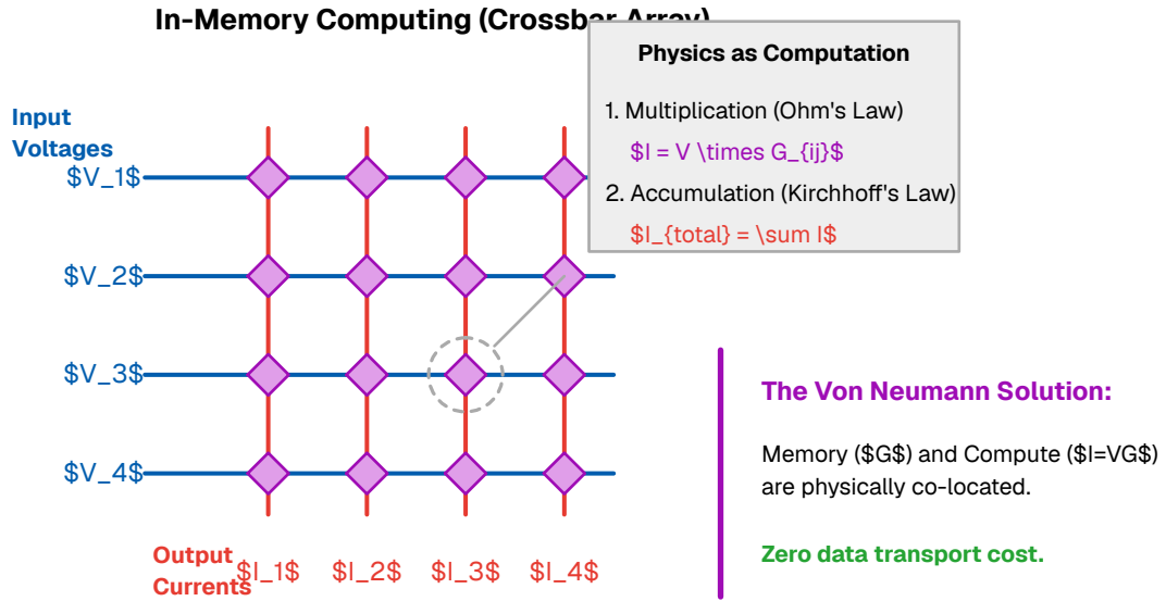
Figure 31: In-Memory Computing via a Crossbar Array. Unlike von Neumann architectures, memory and computation are physically co-located. Input voltages ( V , representing activations) are applied to the wordlines. The memory elements at the junctions hold programmable conductances ( G , representing synaptic weights). Multiplication is naturally performed at each junction by Ohm's Law ( I = V \times G ), and the resulting currents are summed along the bitlines via Kirchhoff's Current Law ( \sum I ). This allows dense matrix-vector multiplications to occur in a single analog time step with zero data transport cost.
