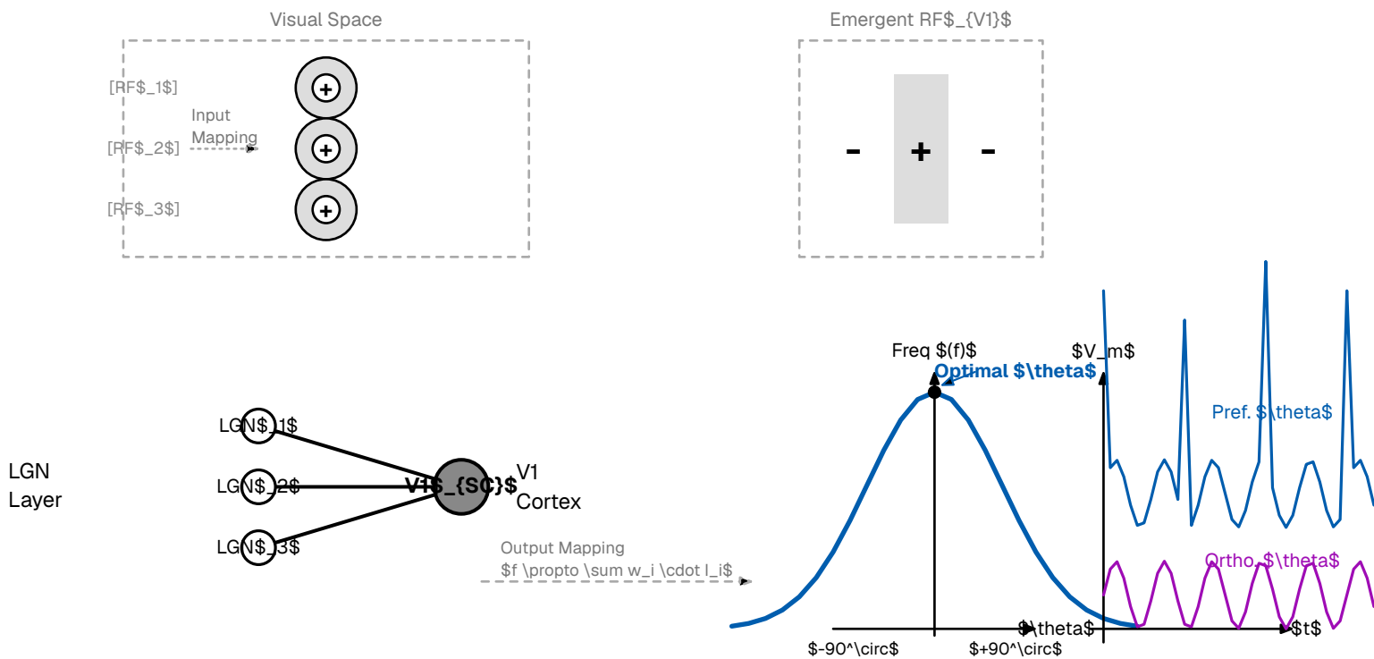
Figure 22: The Hubel & Wiesel Model. Outputs from distinct Retinal/LGN cells converge to form V1 Simple Cells, creating orientation-selective edge detectors.
