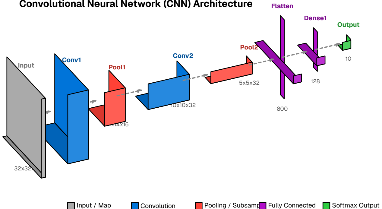
Figure 37: Network architecture for the task at hand
