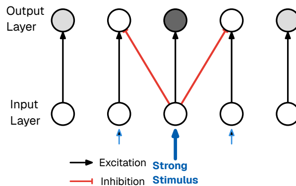
Figure 17: The mechanism of lateral inhibition. (A) A highly stimulated neuron in the input layer strongly excites its corresponding output neuron while simultaneously sending lateral inhibitory signals to its immediate neighbors. (B) This architectural motif acts as a spatial filter, producing a contrast enhancement effect. A broad input stimulus (dashed blue line) is transformed into a sharper output response (solid purple line) characterized by an amplified center and suppressed surroundings (a “Mexican hat” profile), thereby sharpening signal boundaries.
