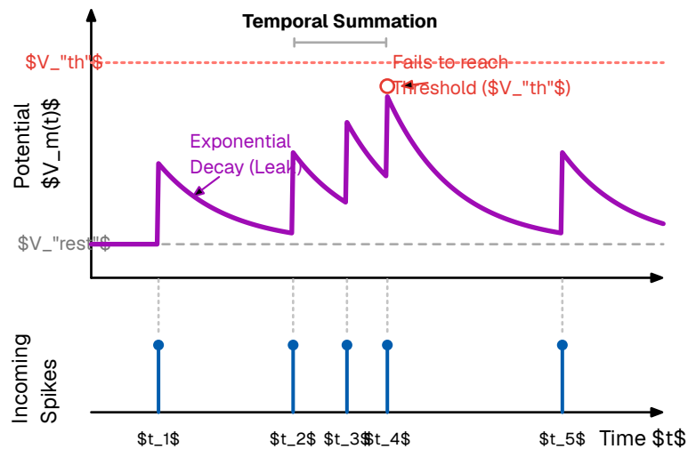
Figure 35: Neuron model where new incoming spikes have an exponential decaying influence on the potential
