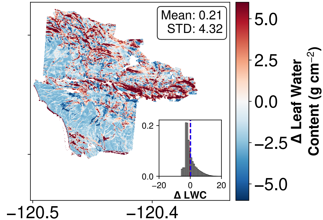
(c) Leaf Water Content
