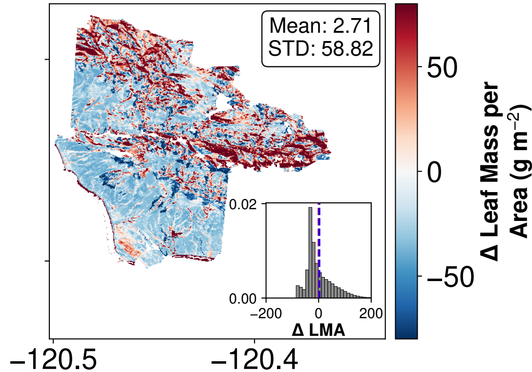
(b) Leaf Mass per Area
