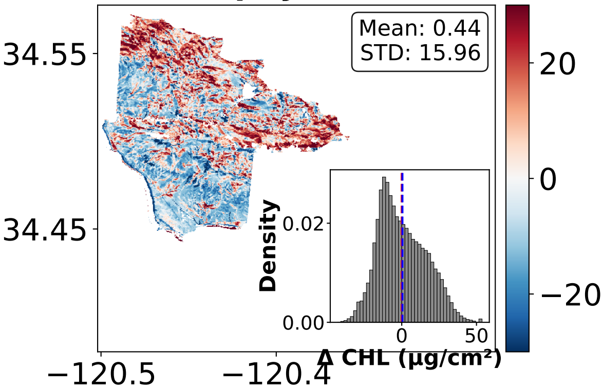
(a) Chlorophyll Content
