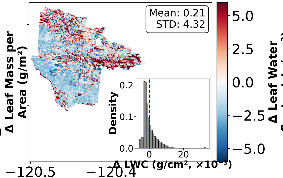
(c) Leaf Water Content ( \times 10^{-3} )
