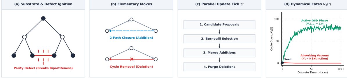
Figure 3: Microscopic graph rewrite system, elementary moves, execution scheduler, and bifurcating dynamical fates. (a) Regular bipartite Bethe substrate ( k = 3 ) with alternating depth-parity node coloring (dark for even depths, open for odd depths) and an initial parity-breaking defect edge linking inner same-parity nodes. (b) Elementary rewrite moves: path-closing addition on directed 2-paths and tension-dependent deletion on 3-cycle edges under causal PUC and AEC constraints. (c) Maximally parallel discrete tick \mathcal{U} executing candidate proposals, independent Bernoulli selections, idempotent addition merge, and deletion purge (Lemma 4.6.1). (d) Dynamical trajectories of 3-cycle population N_3(t) , illustrating the bifurcation between rapid decay to the frozen absorbing vacuum ( N_3 = 0 ) and first-tick burst escape into a persistent Quasi-Stationary Distribution (QSD, \langle N_3 \rangle_{\text{QSD}} \approx 124 at N = 10^4 ).
