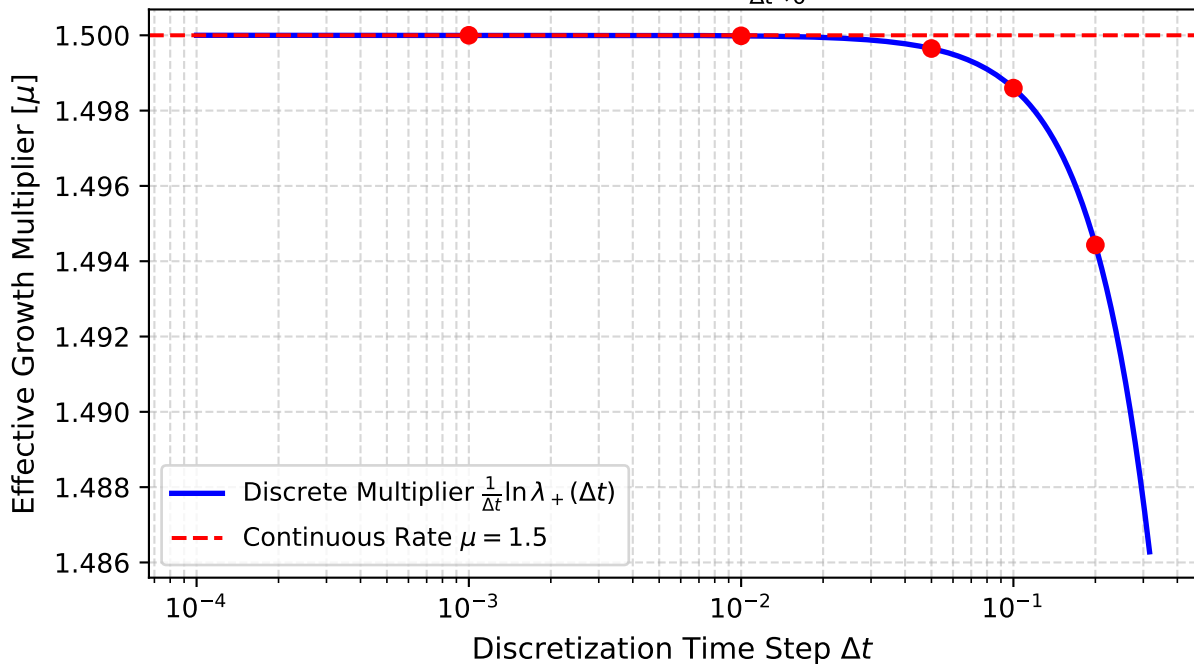
(b) Continuum Limit: \lim_{\Delta t \rightarrow 0} \frac{1}{\Delta t} \ln \lambda_+ = \mu
