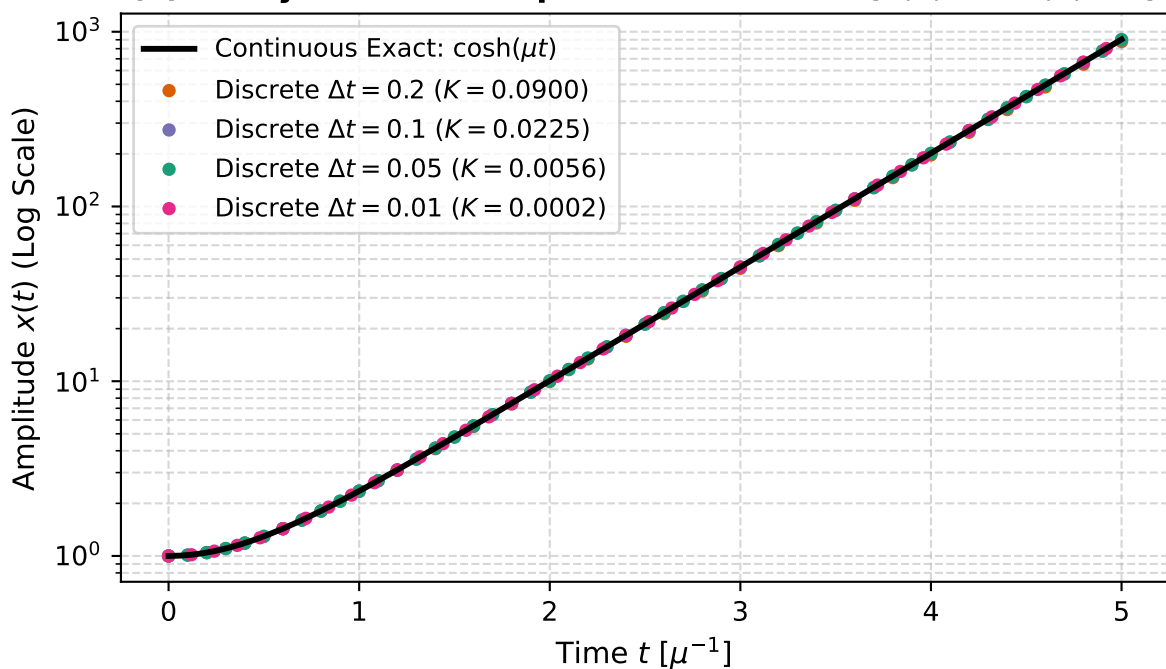
(a) Tachyonic Mode Explosion from Rest ( x(0) = 1, \dot{x}(0) = 0 )
