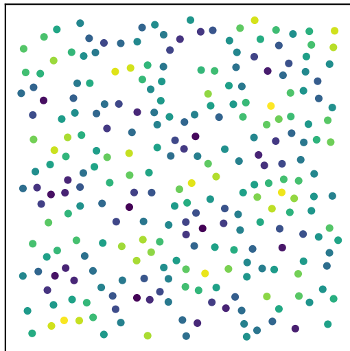
LF-pretrained (L2=1.48%)
