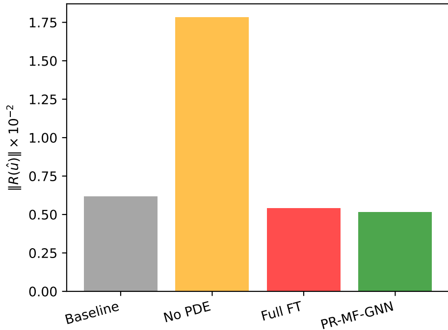
PDE Residual
