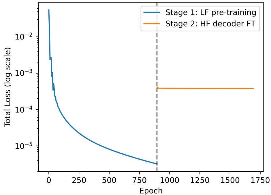
Training Loss
