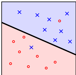
Simple model: 89% of training points
