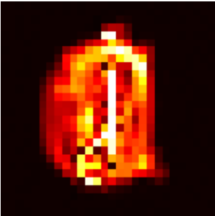
Difference MSE: 0.0239
