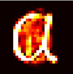
Difference MSE: 0.0570
