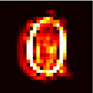
Difference MSE: 0.0342
