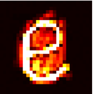
Difference MSE: 0.0485
