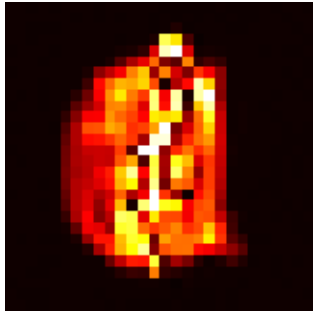
Difference MSE: 0.0218
