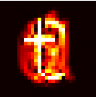
Difference MSE: 0.0280
