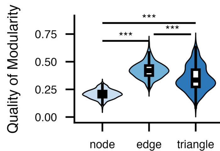
e. Replication Cohort
