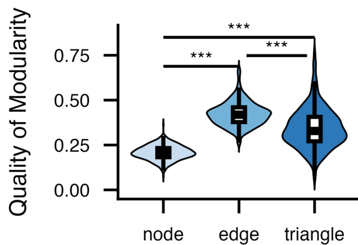
d. Exploration Cohort
