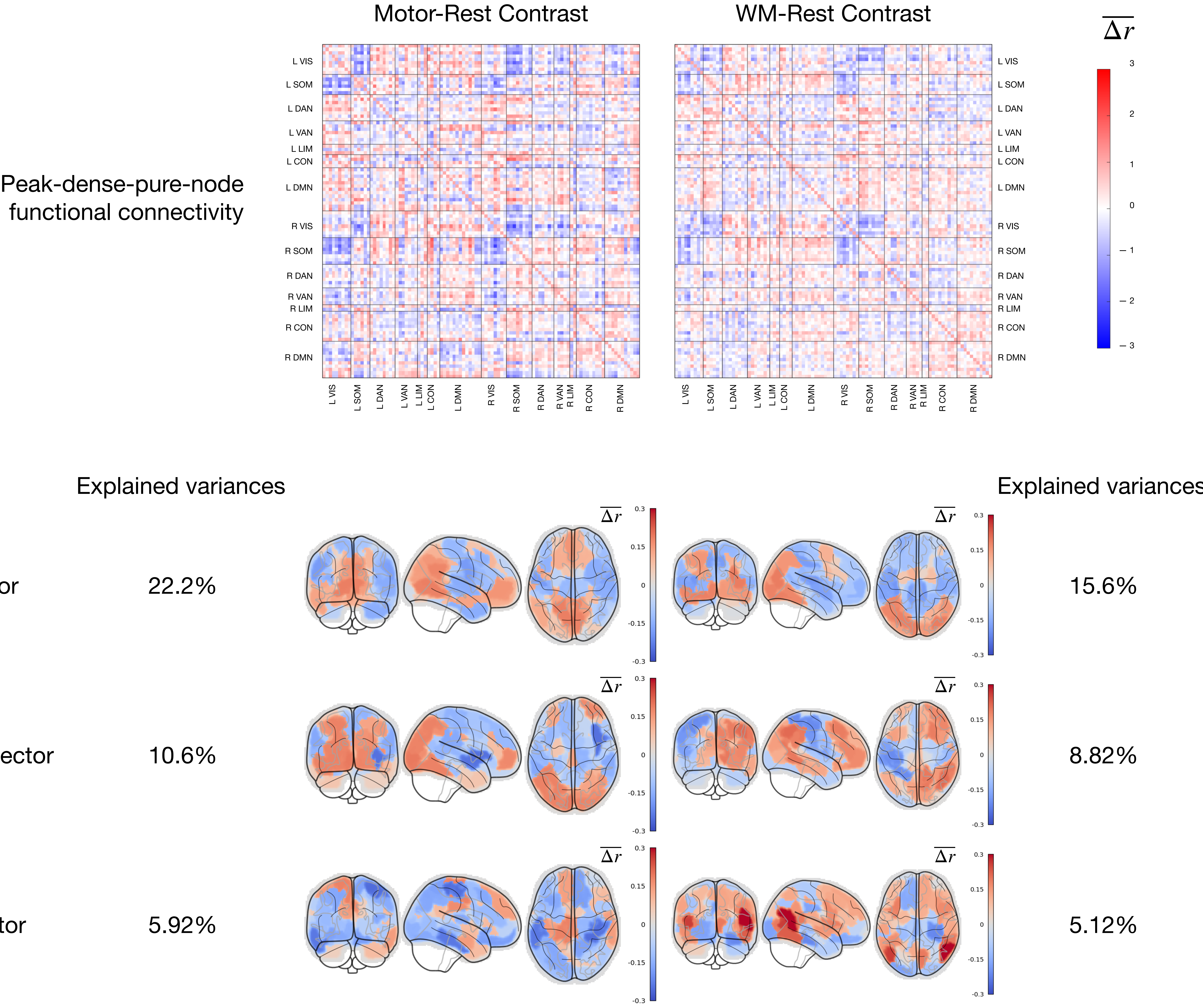
c. Mean Task Frame-Level Peak-Dense-Pure-Node Functional Connectivity and Associated Eigenvectors
