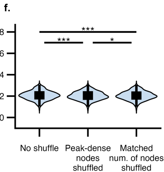
Replication Cohort Quality of Modularity
