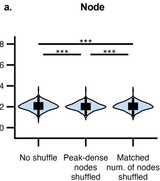
Exploration Cohort Quality of Modularity
