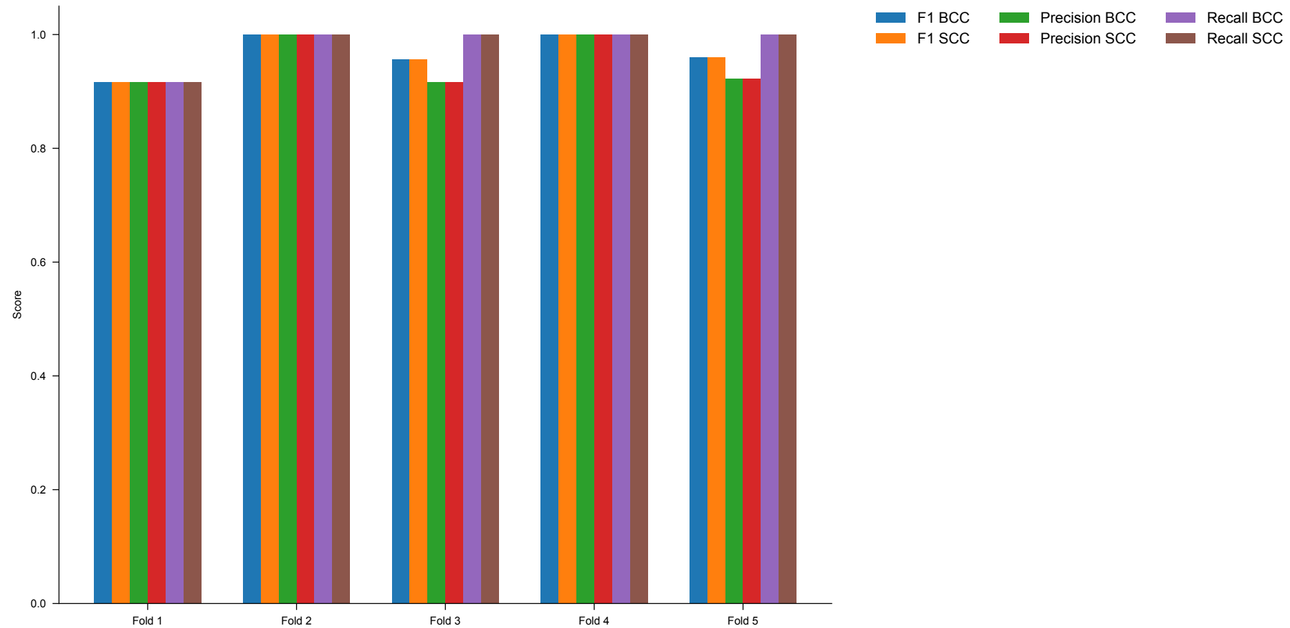
Per-class metrics per fold
