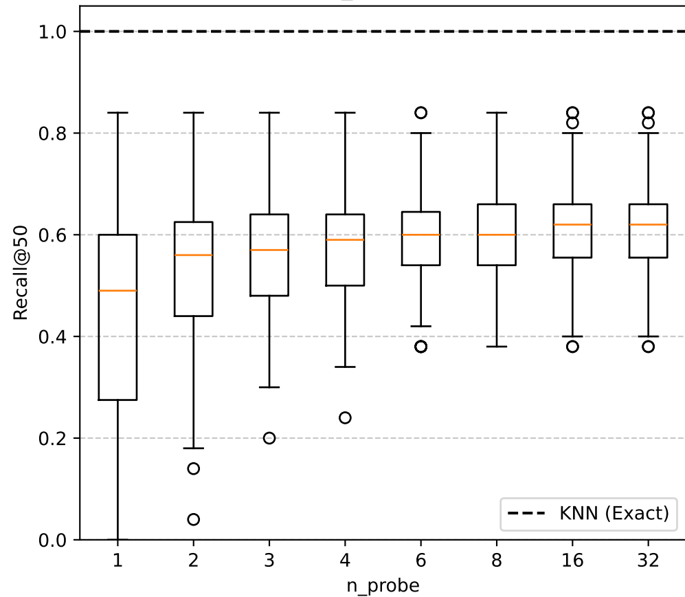
n_{\text{sub}} = 8
