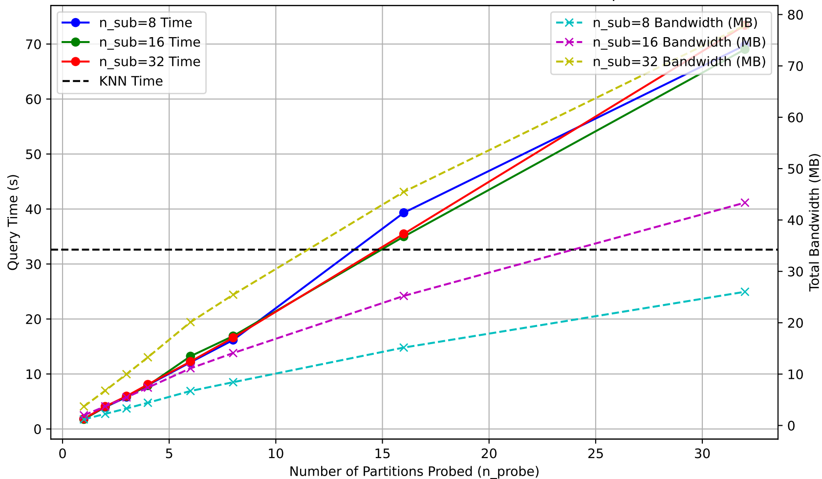
IVFPQ Time and Bandwidth vs. Probes for Different Subspaces
