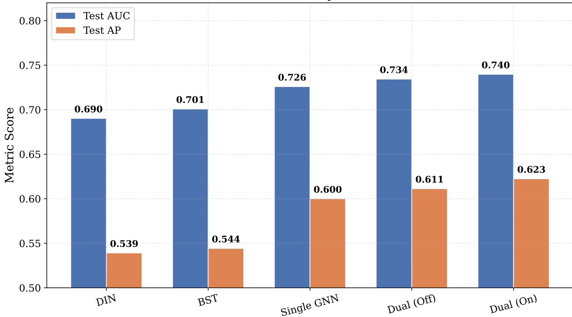
Predictive Accuracy (AUC & AP)
