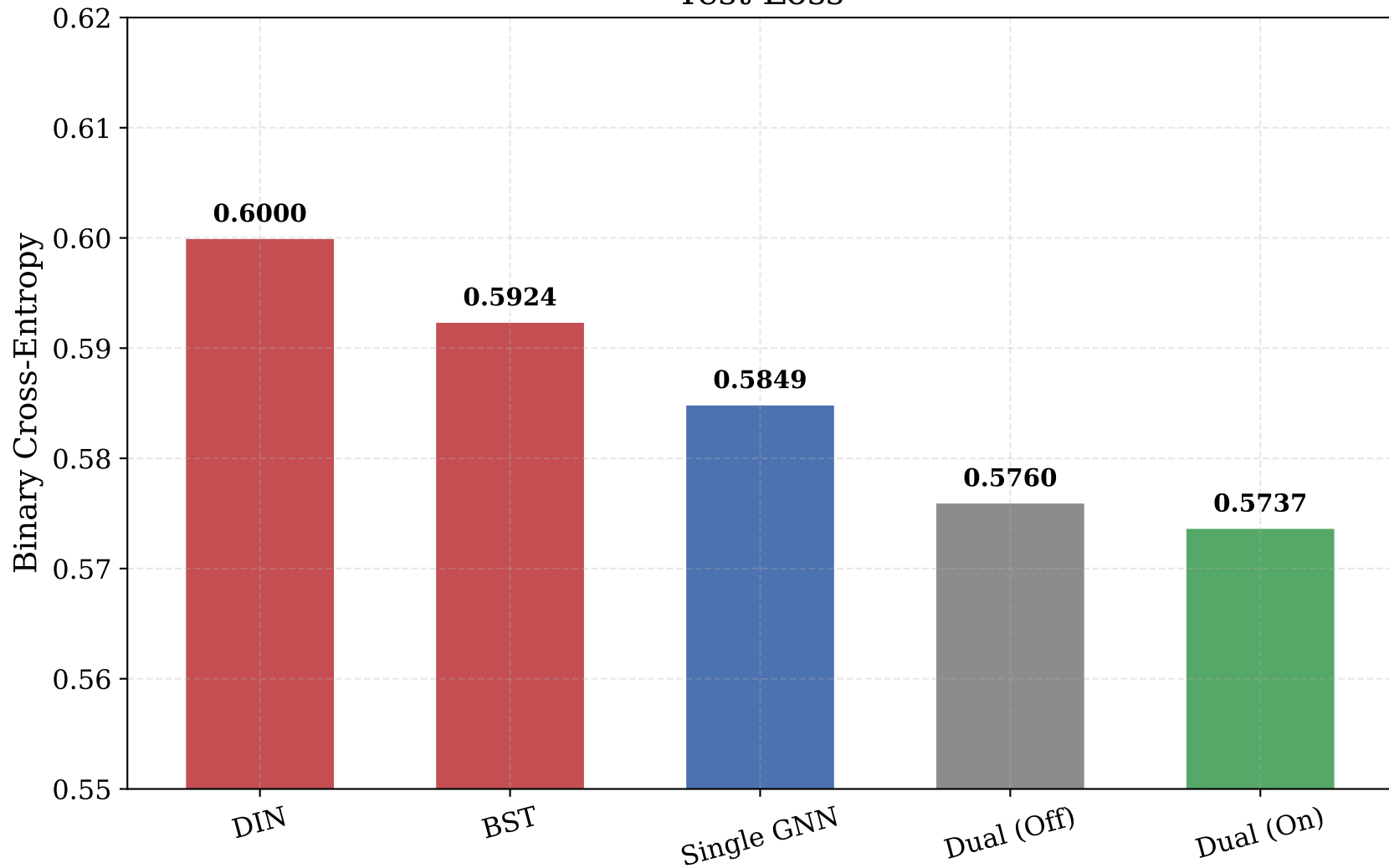
Test Loss
