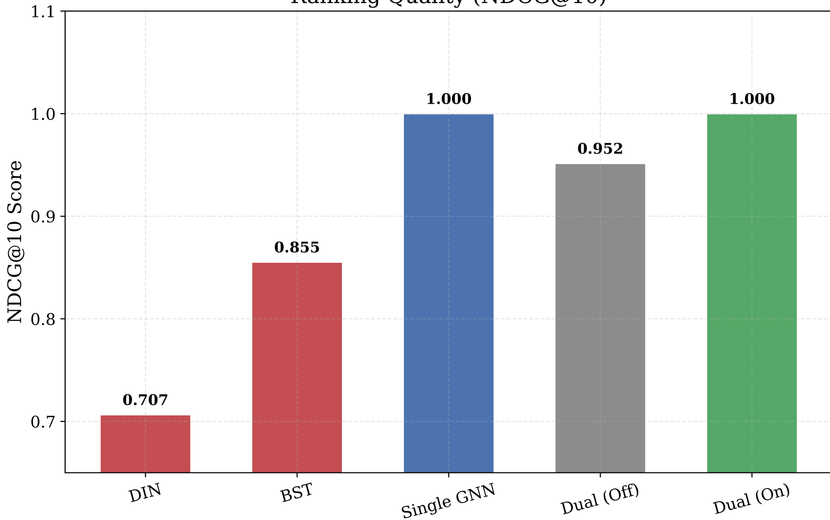
Ranking Quality (NDCG@10)
