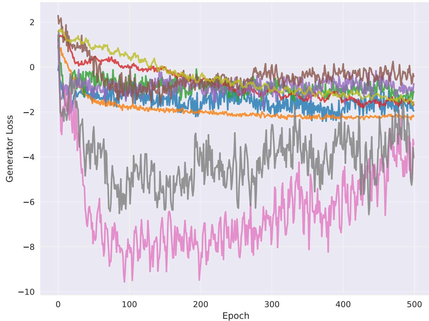
CTGAN Generator Loss by Dataset
