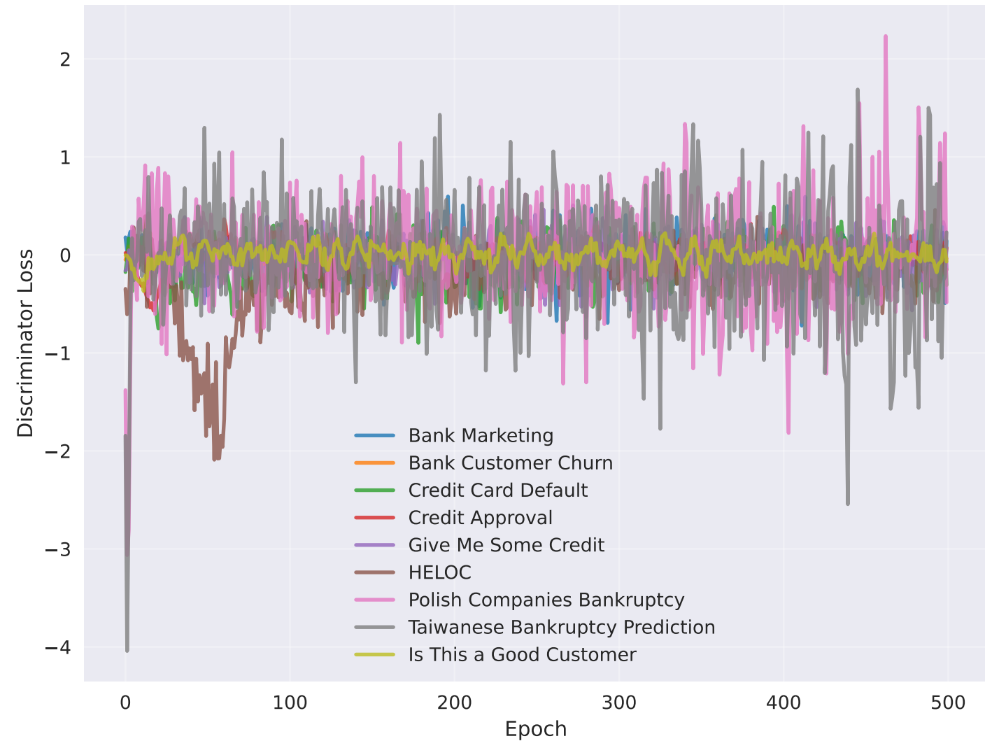
CTGAN Discriminator Loss by Dataset
