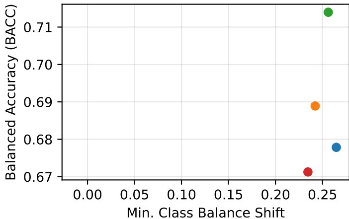
Balanced Labels
