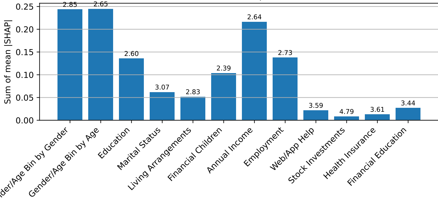
Colorado SHAP Importances
