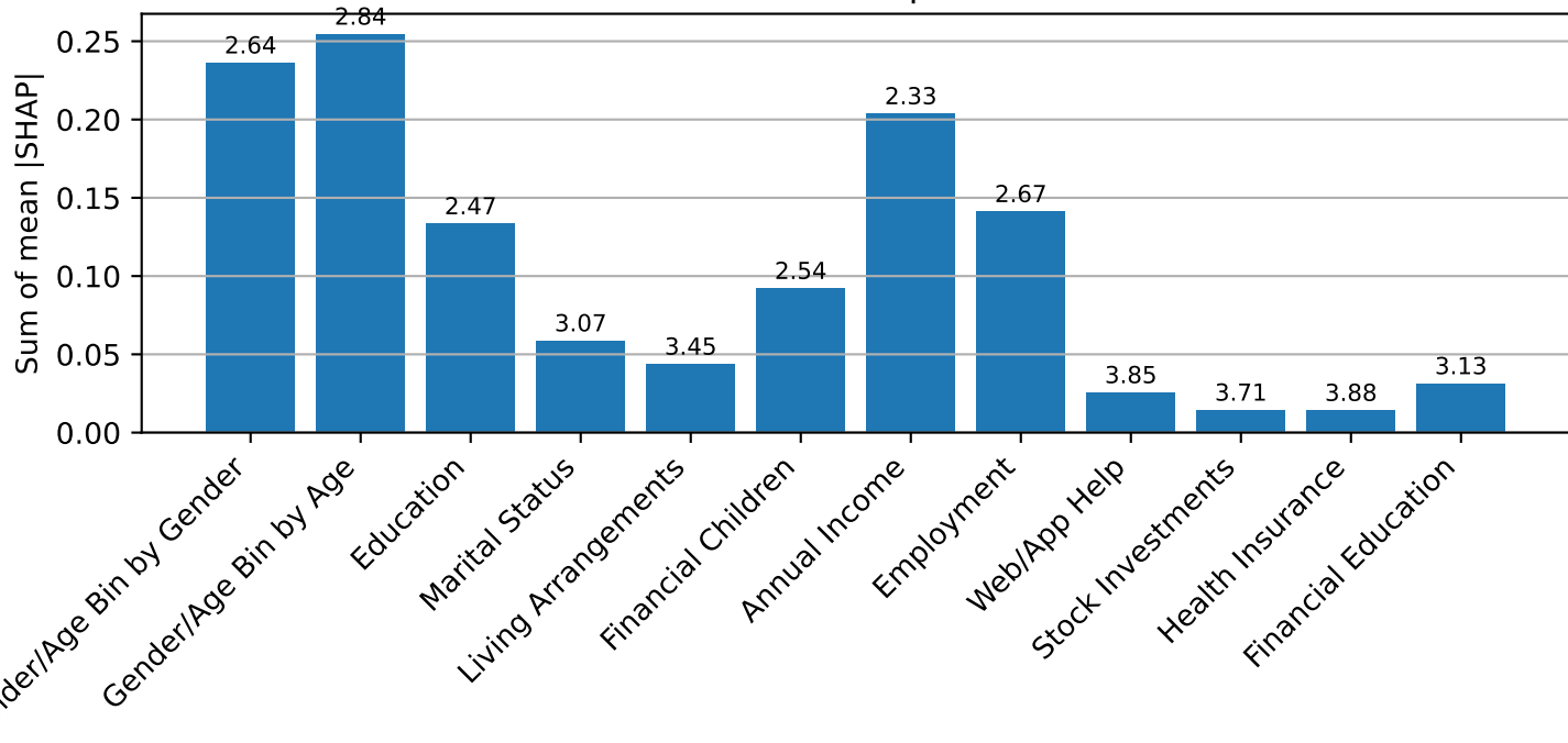
Florida SHAP Importances
