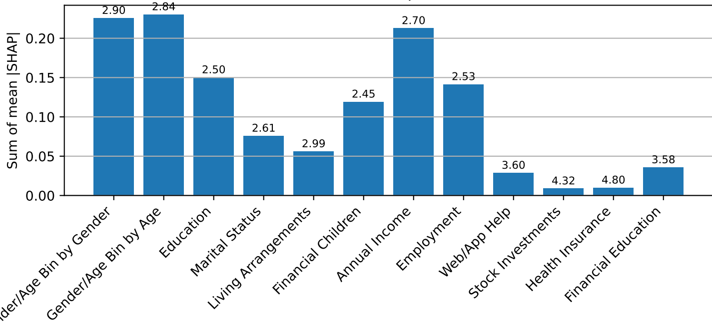
Texas SHAP Importances
