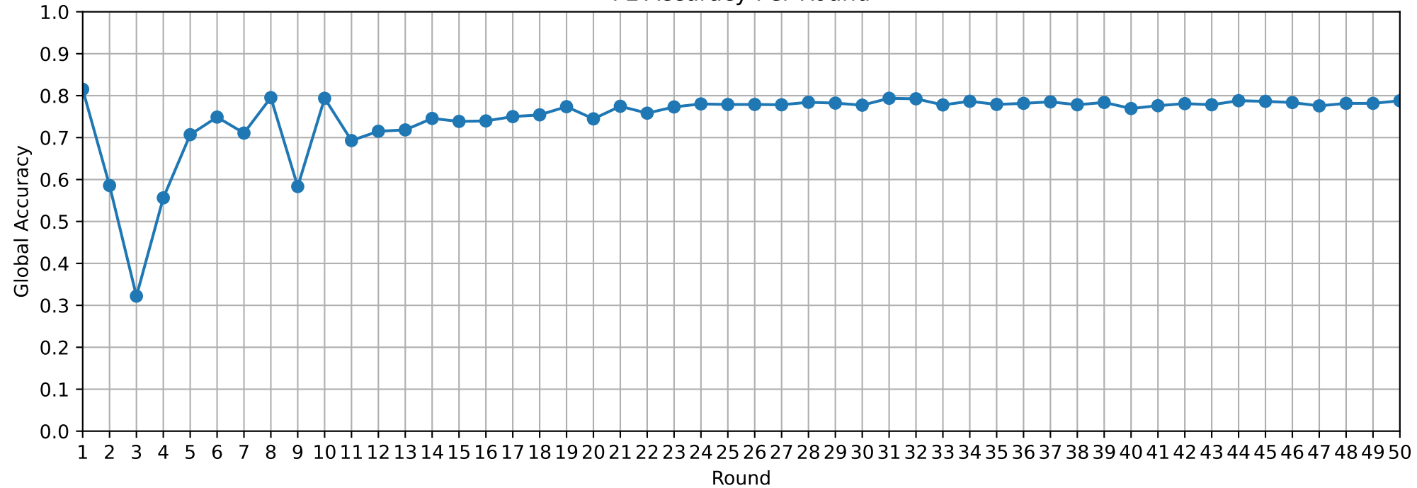
FL Accuracy Per Round
