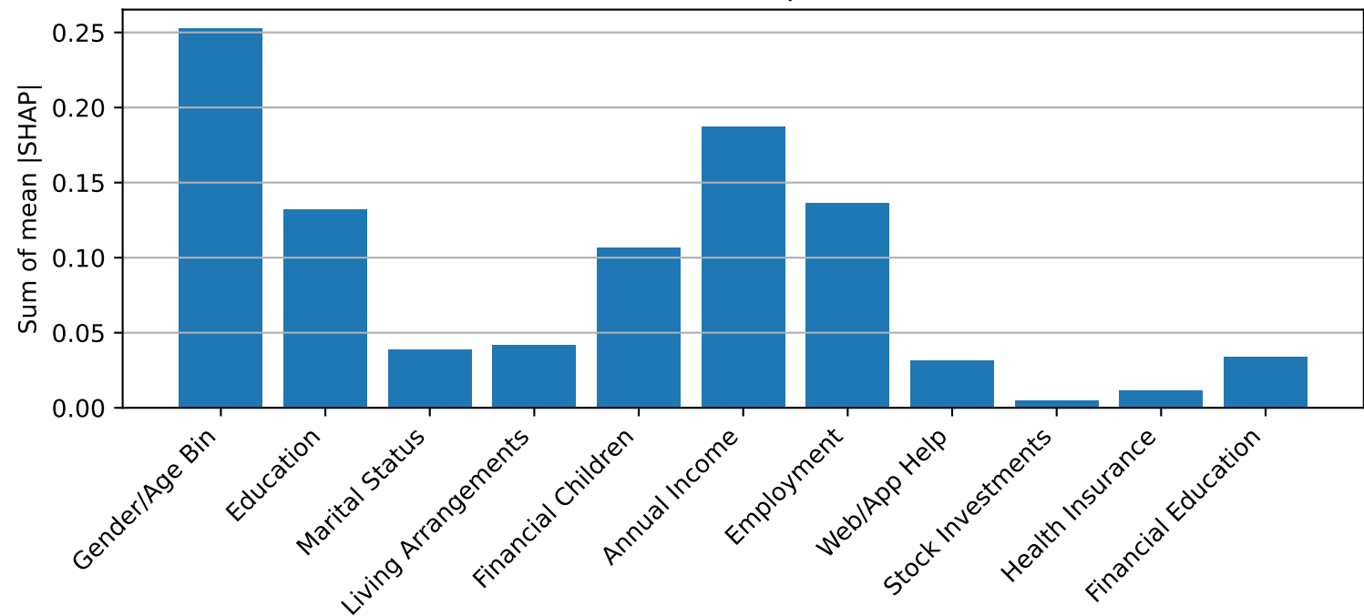
Hawaii SHAP Importances
