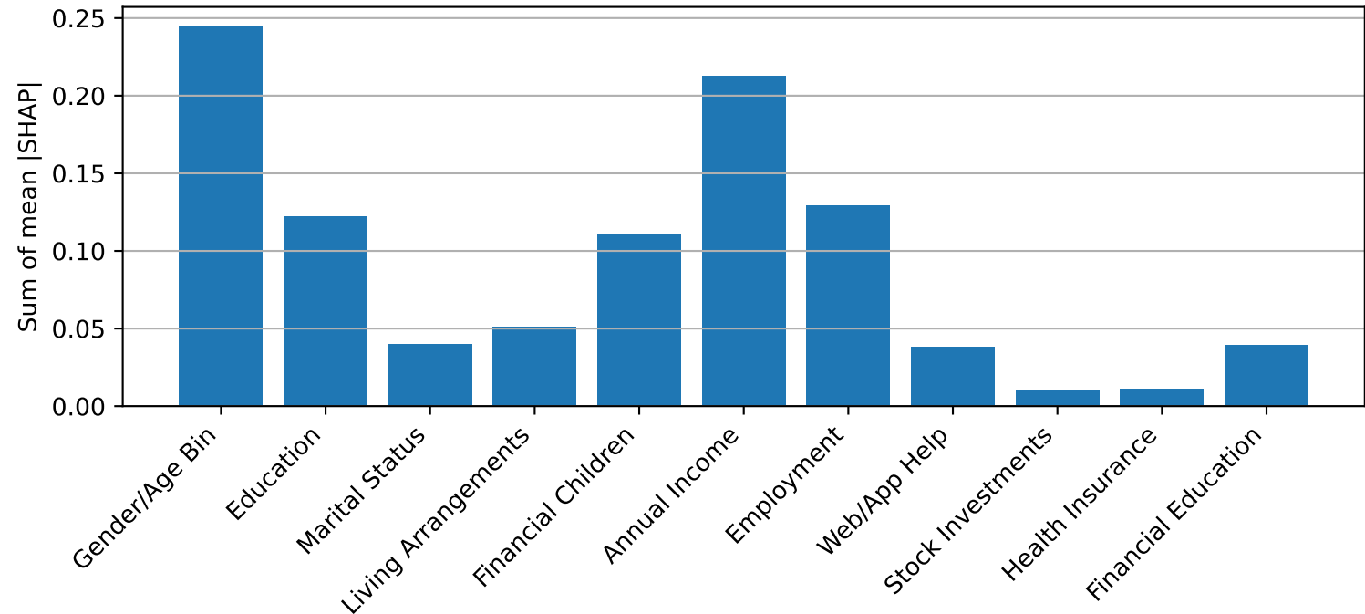
Kansas SHAP Importances
