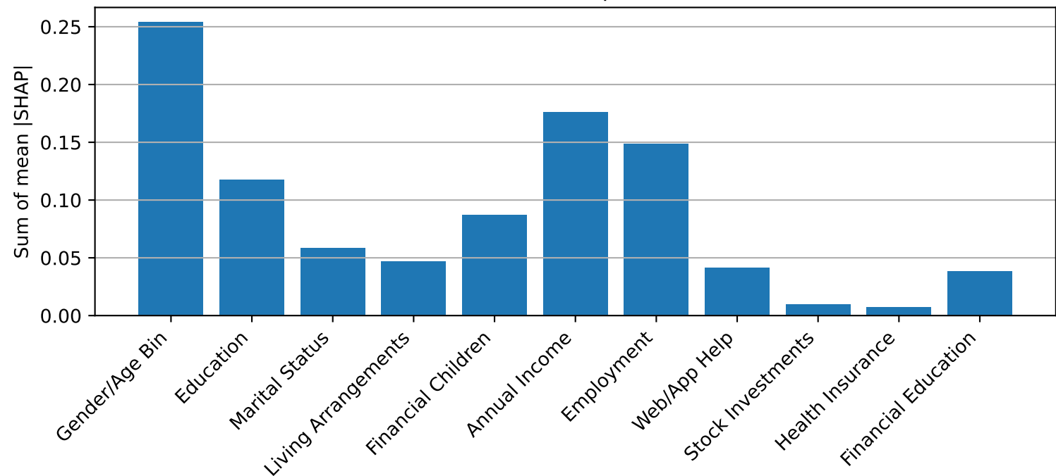
Texas SHAP Importances
