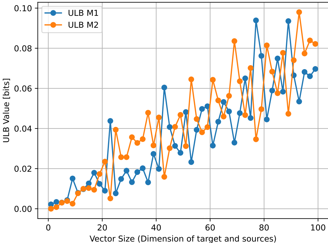
ULB vs Vector Size_both_unique_ULB
