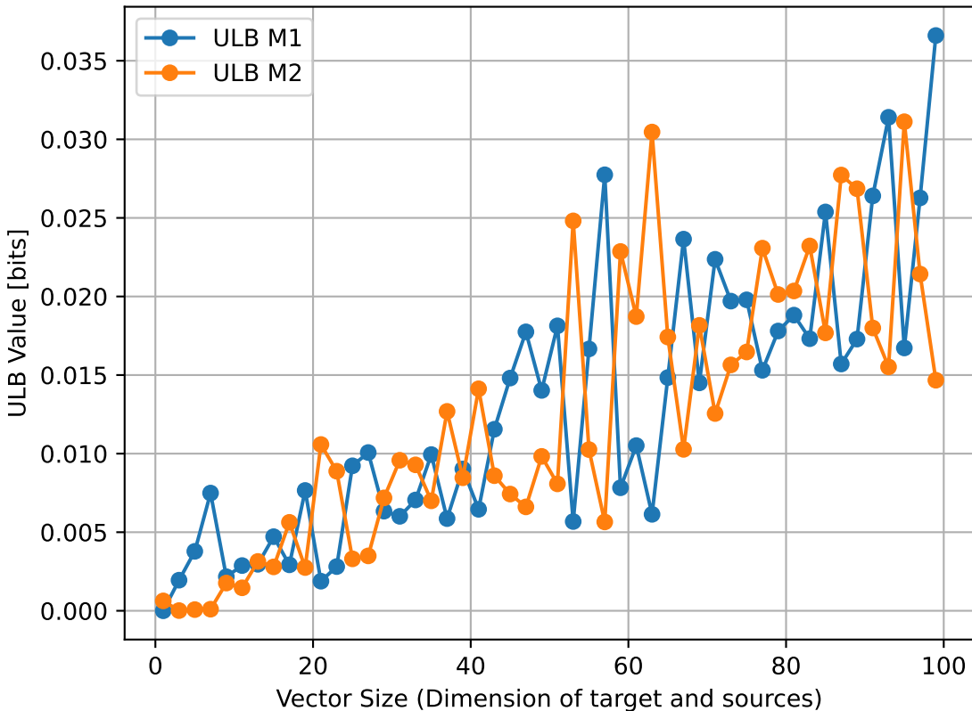
ULB vs Vector Size
