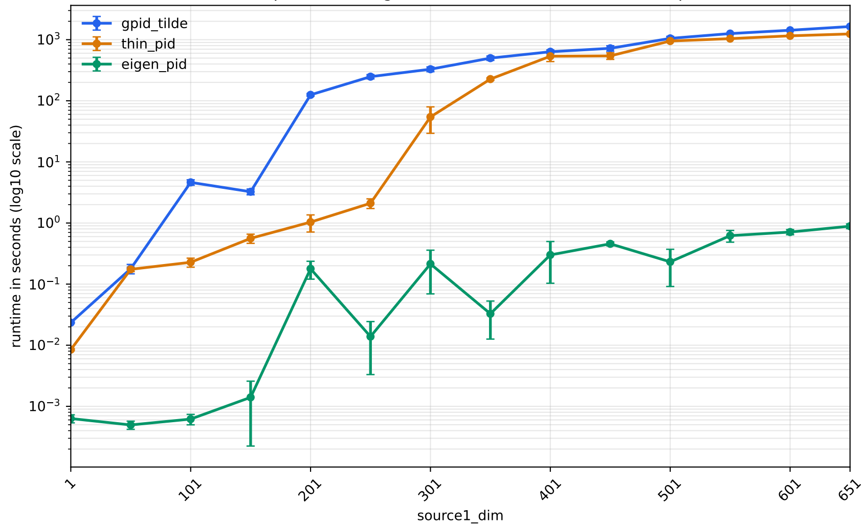
Runtime comparison through dimension 651 (mean \pm SD; 5 repetitions)
