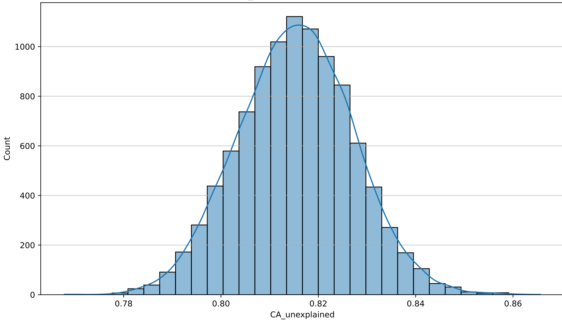
CA_unexplained distribution
